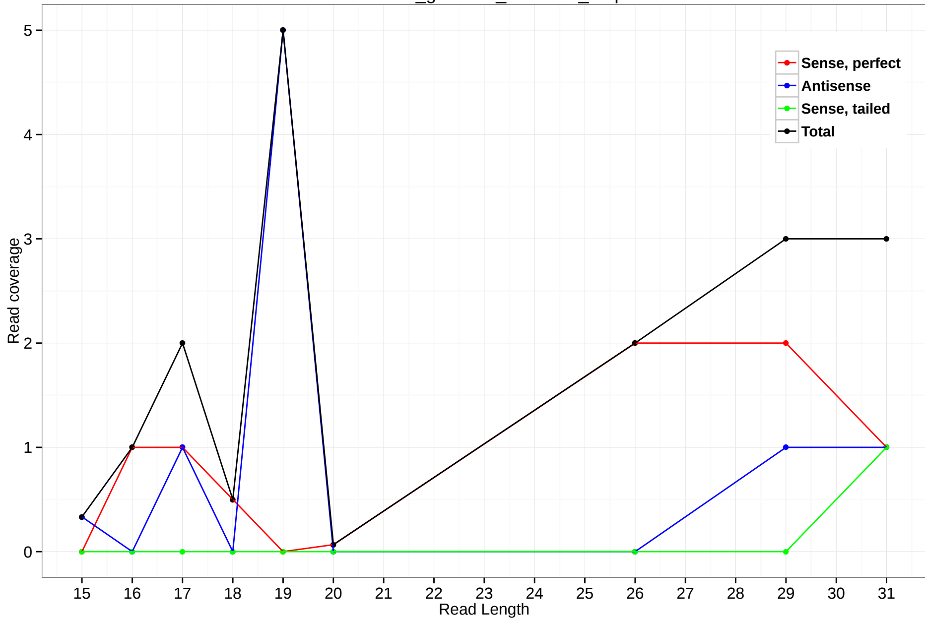
rheMac3_genscan_chr7.948_1.3p
