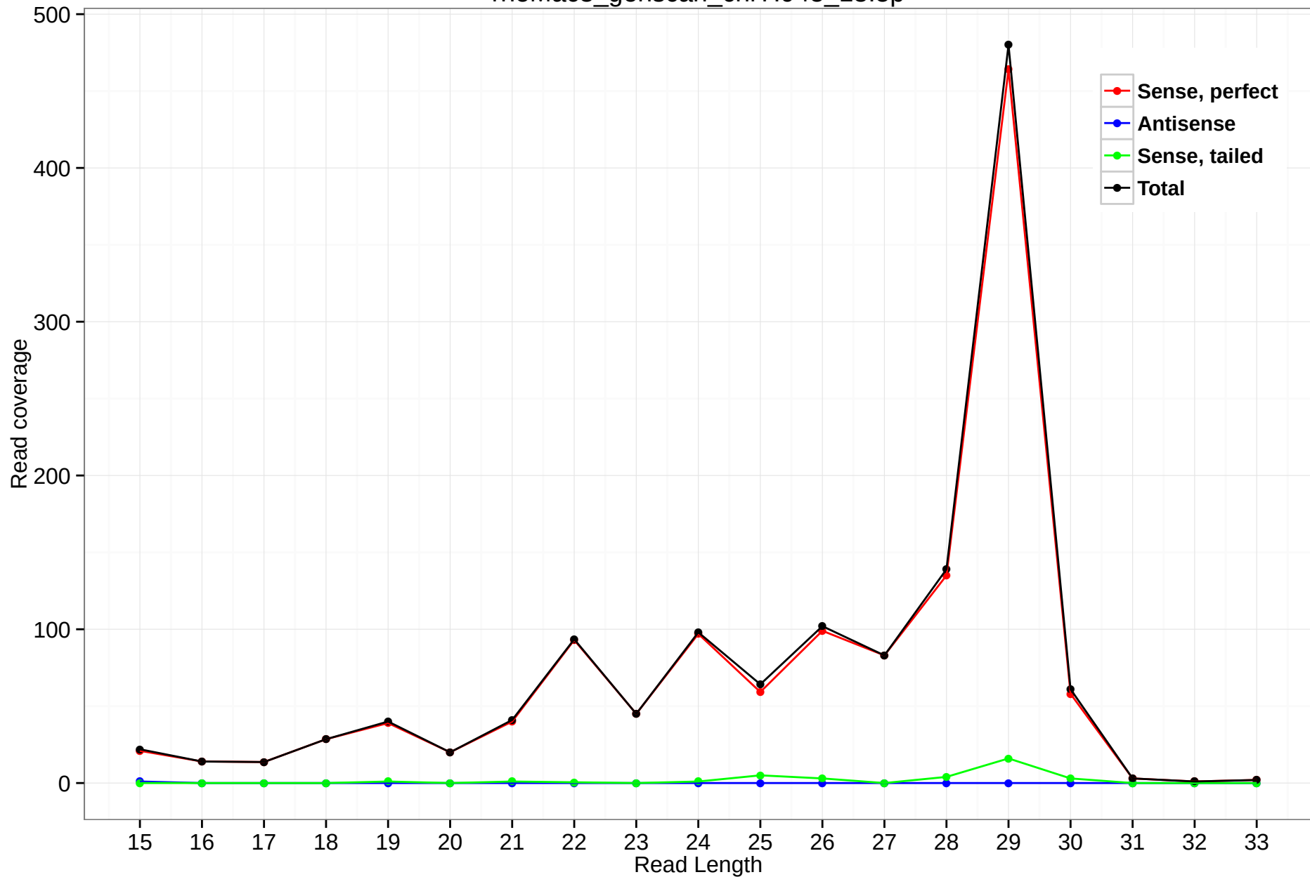
rheMac3_genscan_chr7.945_18.5p
