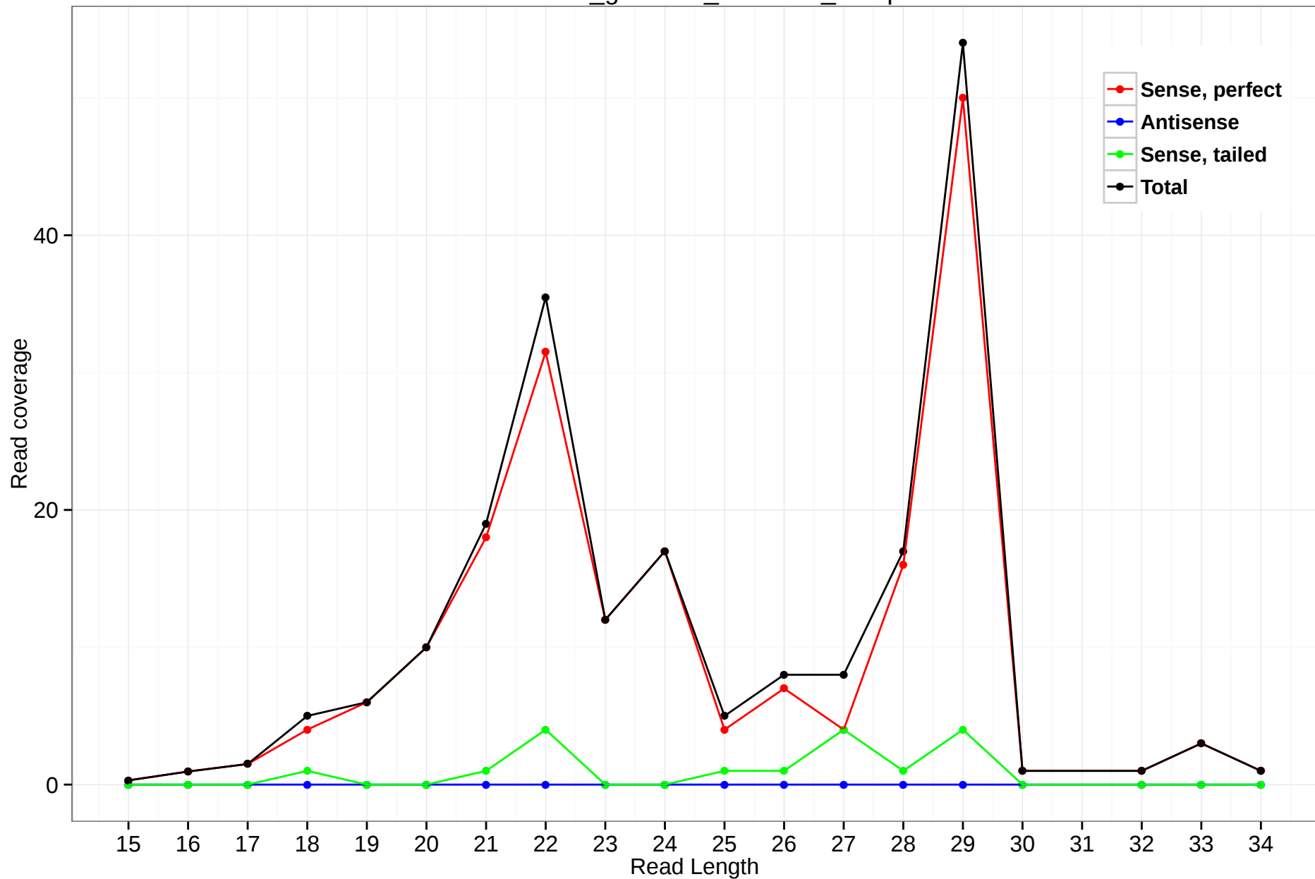
rheMac3_genscan_chr7.945_18.3p
