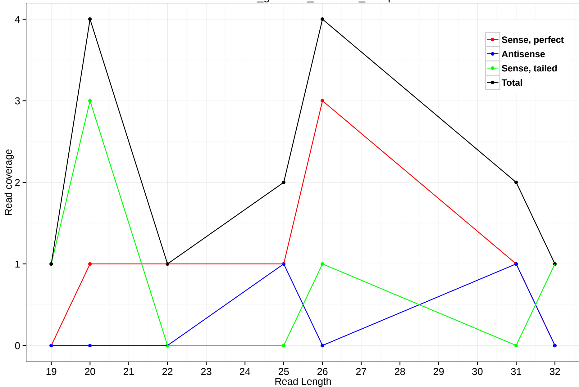
rheMac3_genscan_chr7.900_15.3p
