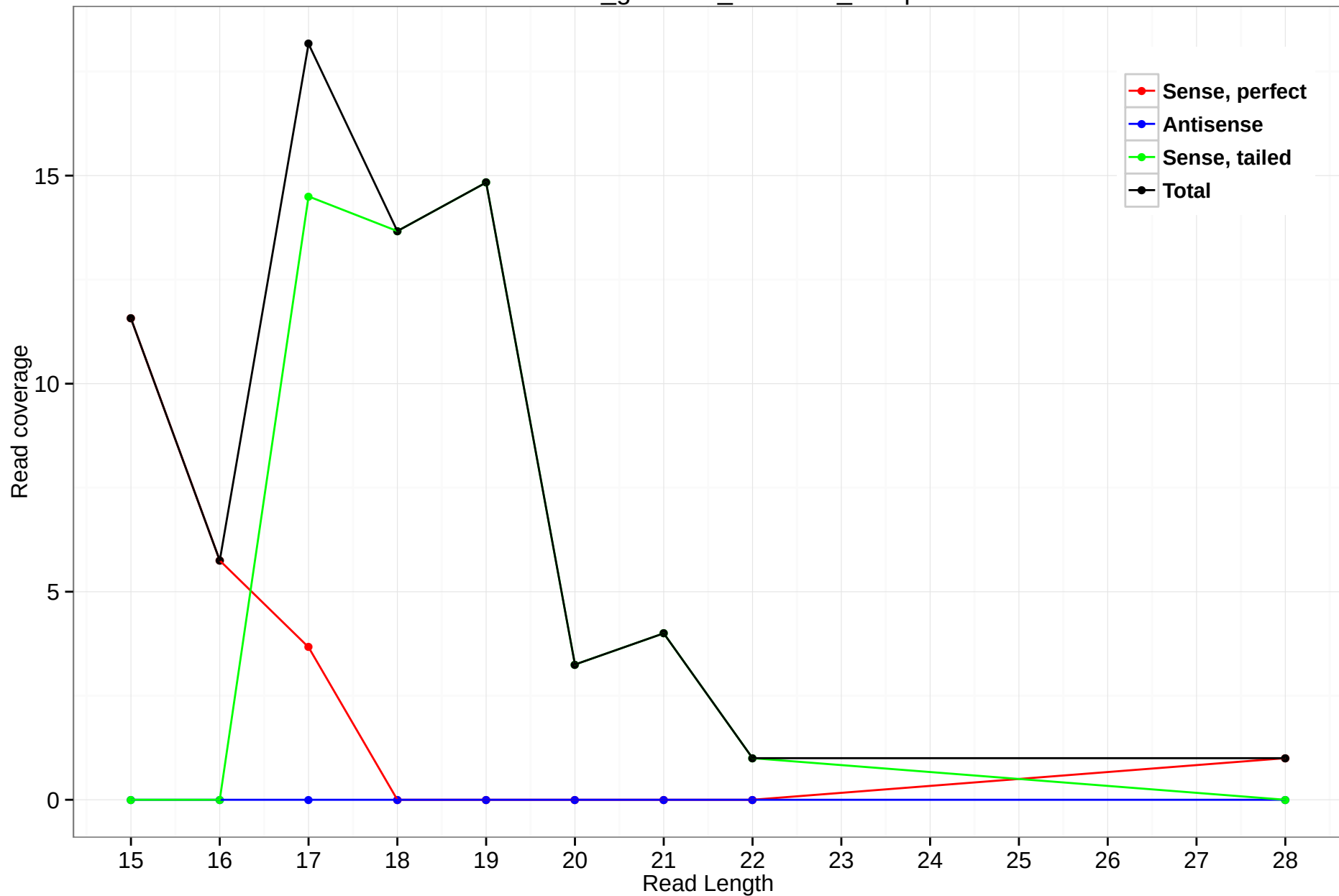
rheMac3_genscan_chr7.872_38.5p
