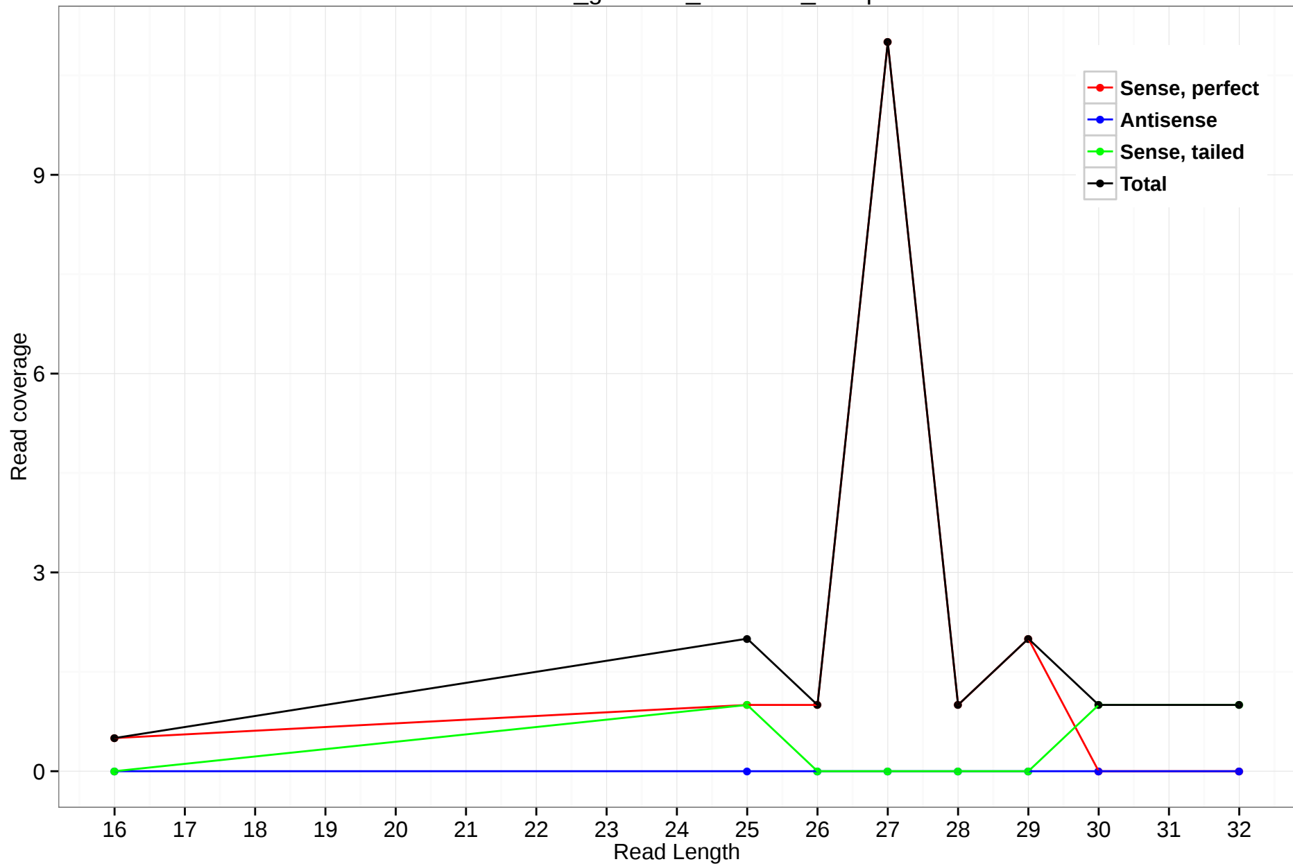
rheMac3_genscan_chr7.842_46.3p
