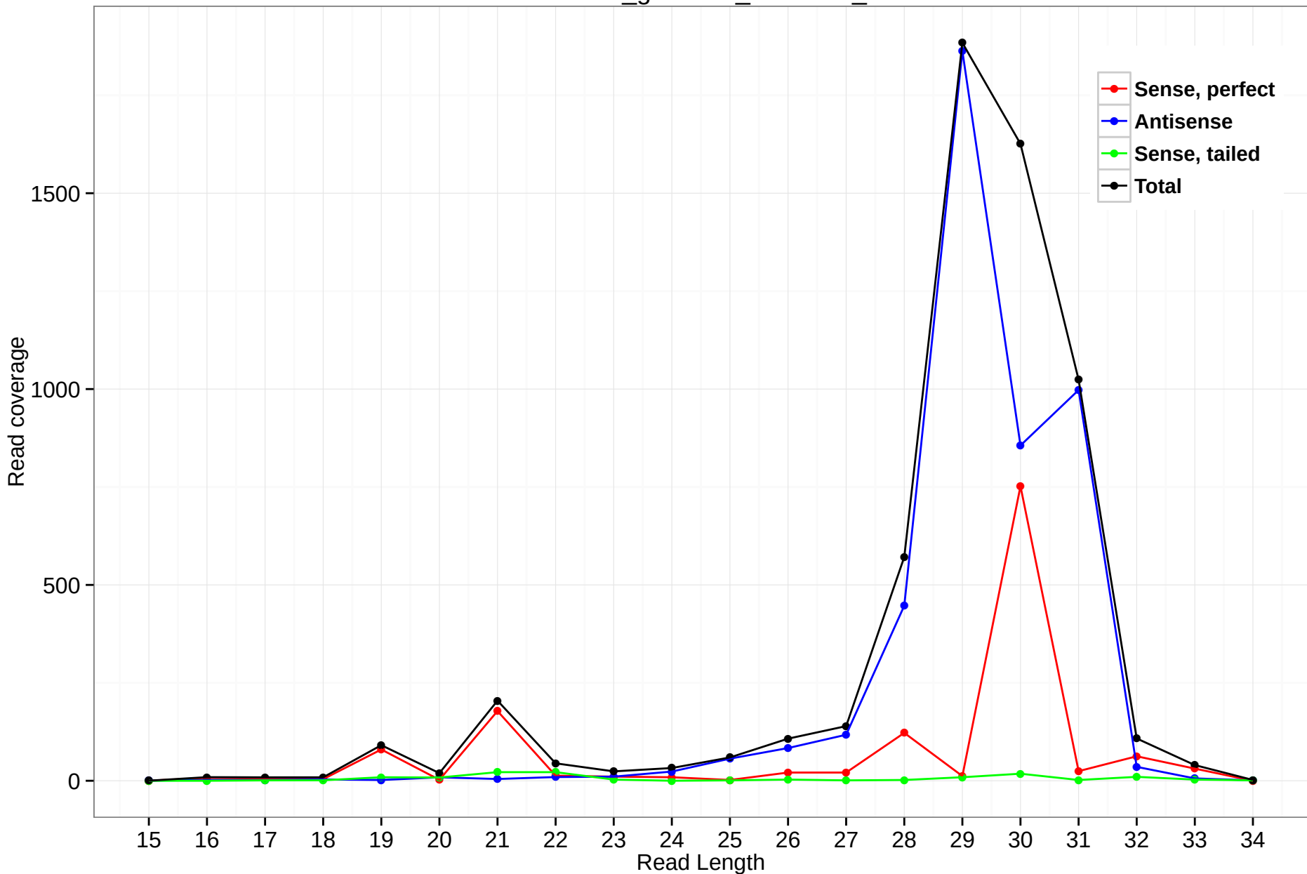
rheMac3_genscan_chr7.829_9
