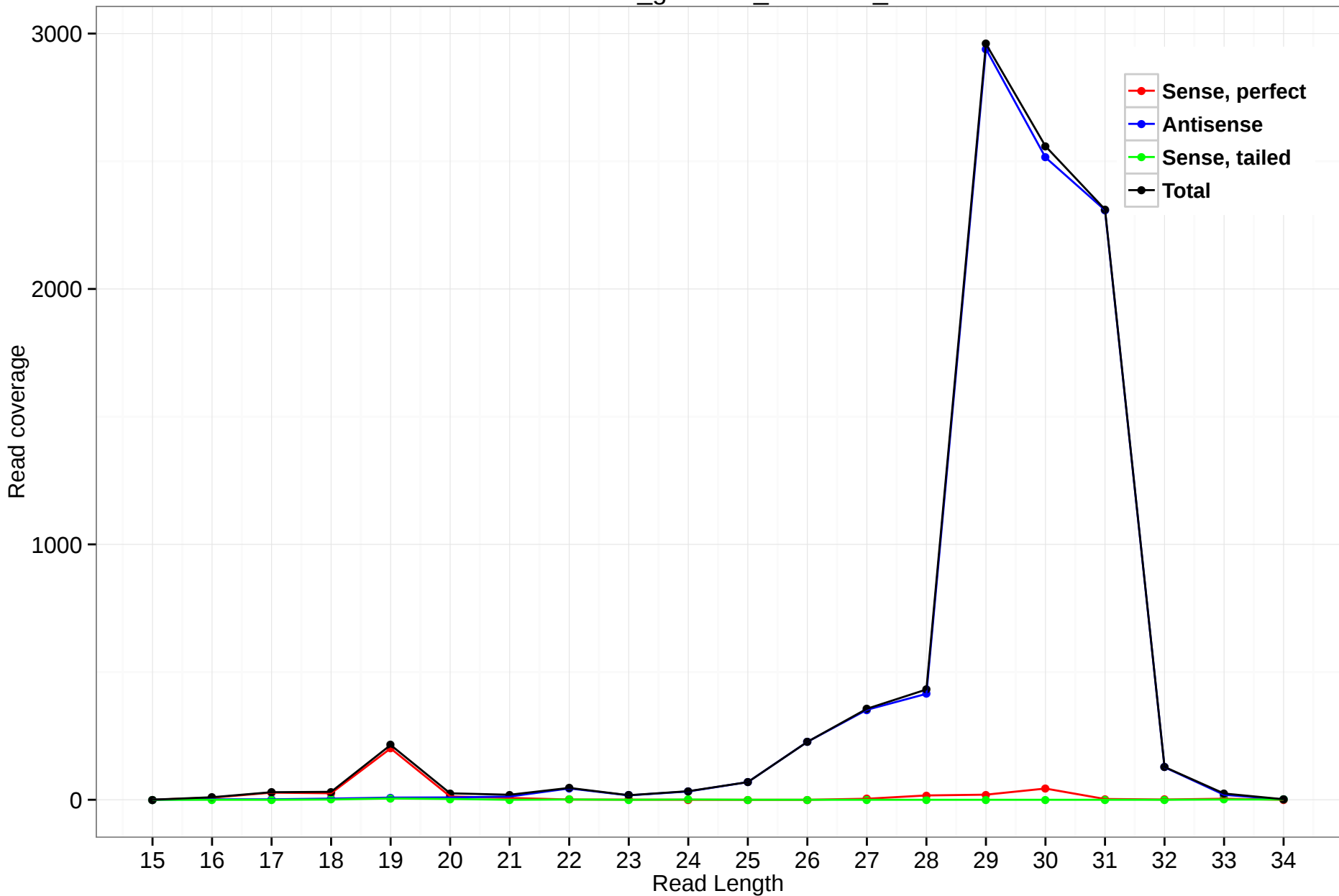
rheMac3_genscan_chr7.829_6
