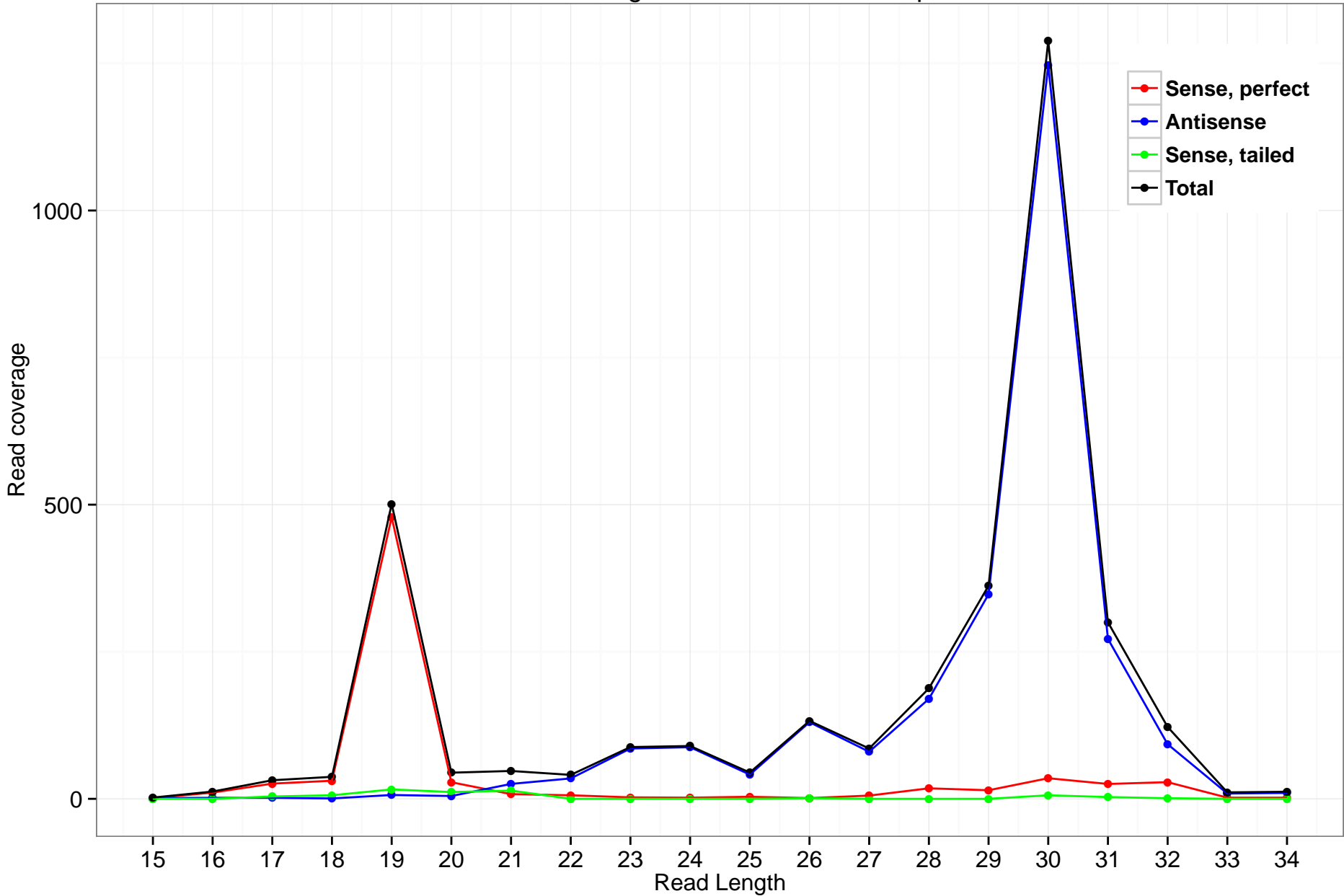
rheMac3_genscan_chr7.829_27.3p
