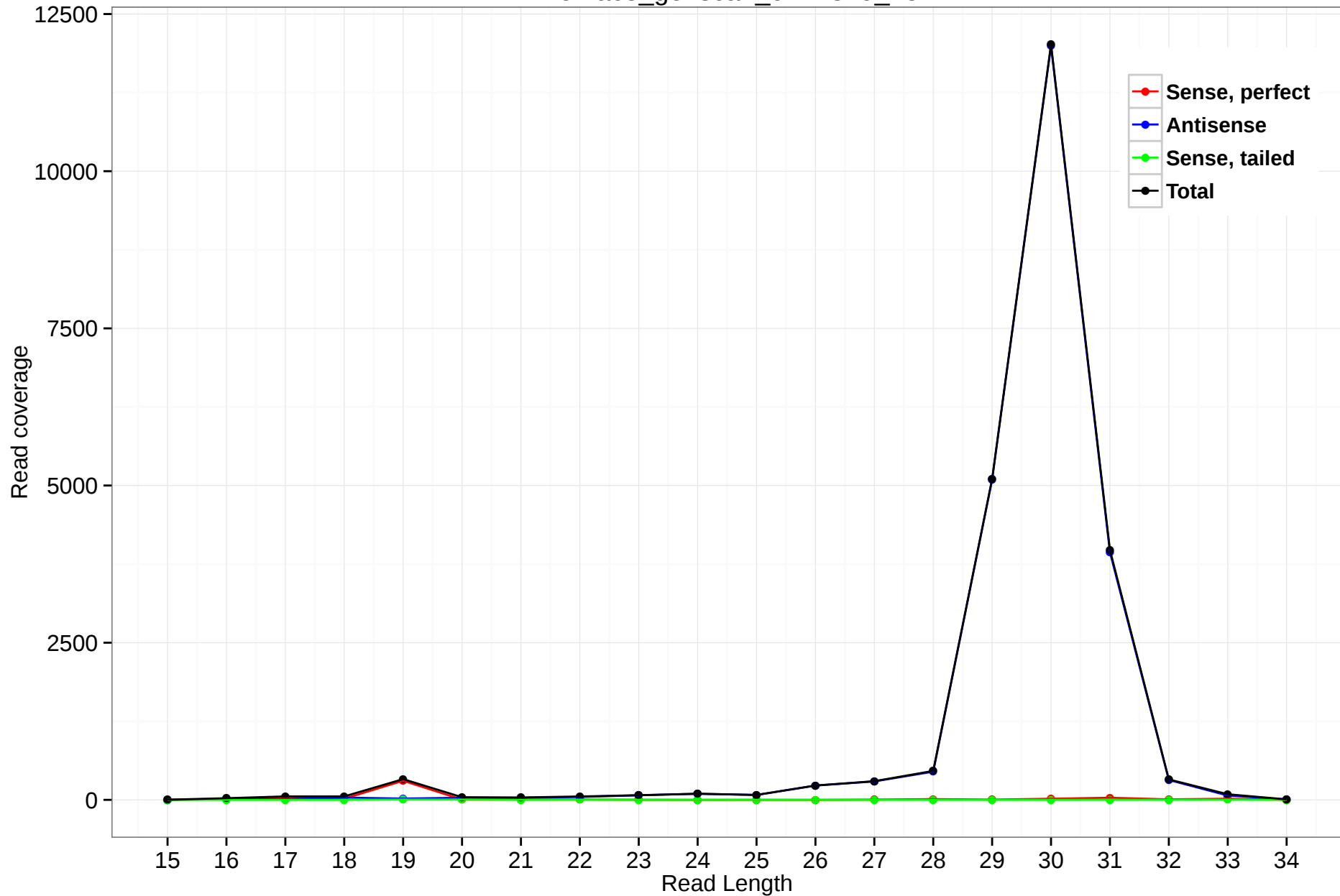
rheMac3_genscan_chr7.829_25
