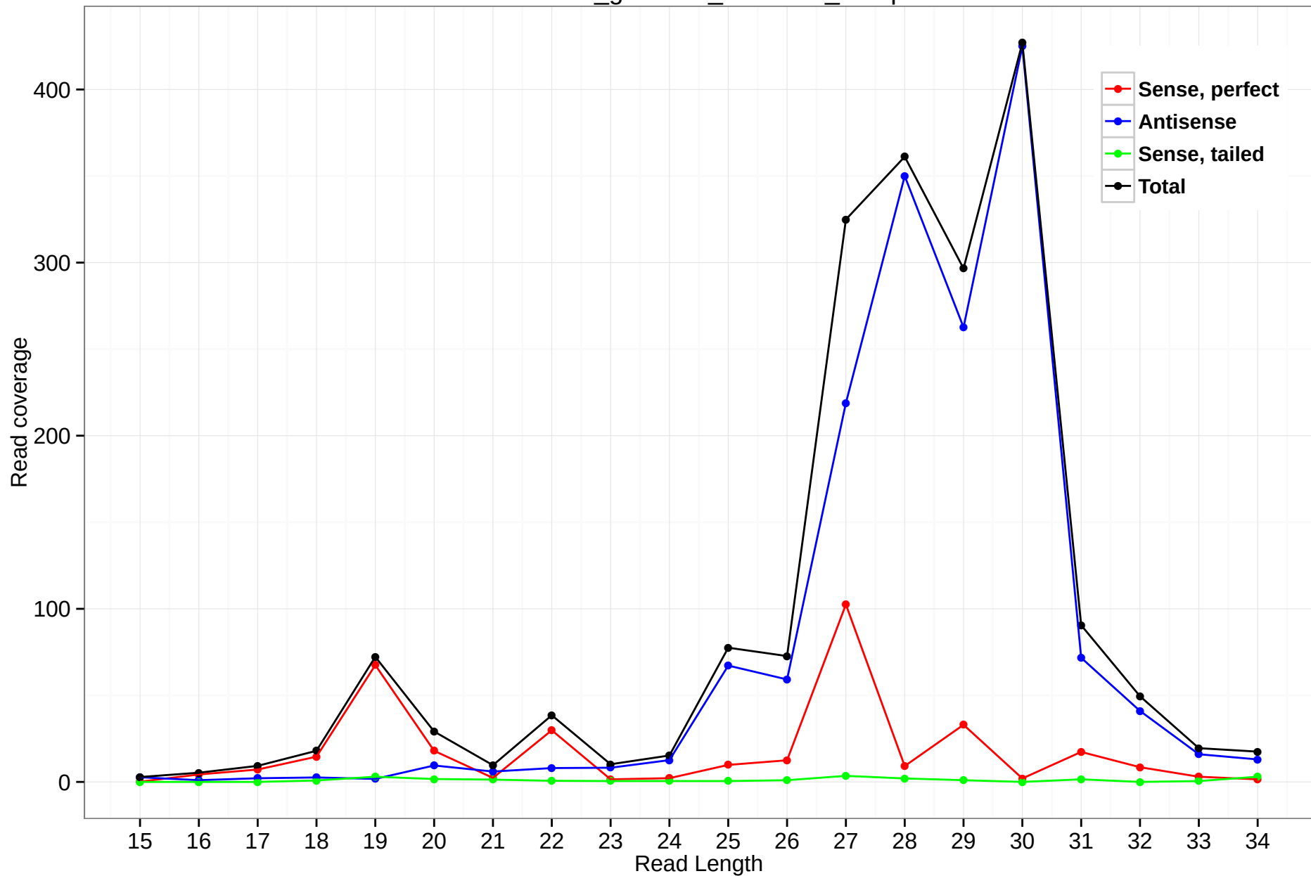
rheMac3_genscan_chr7.829_23.3p
