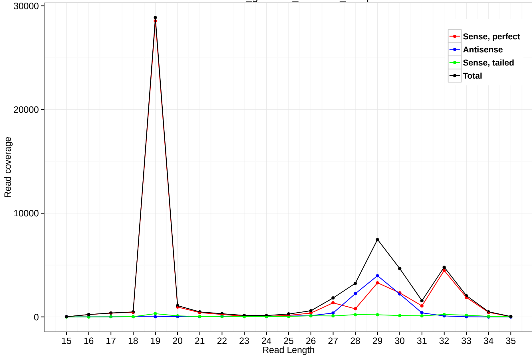
rheMac3_genscan_chr7.829_22.3p
