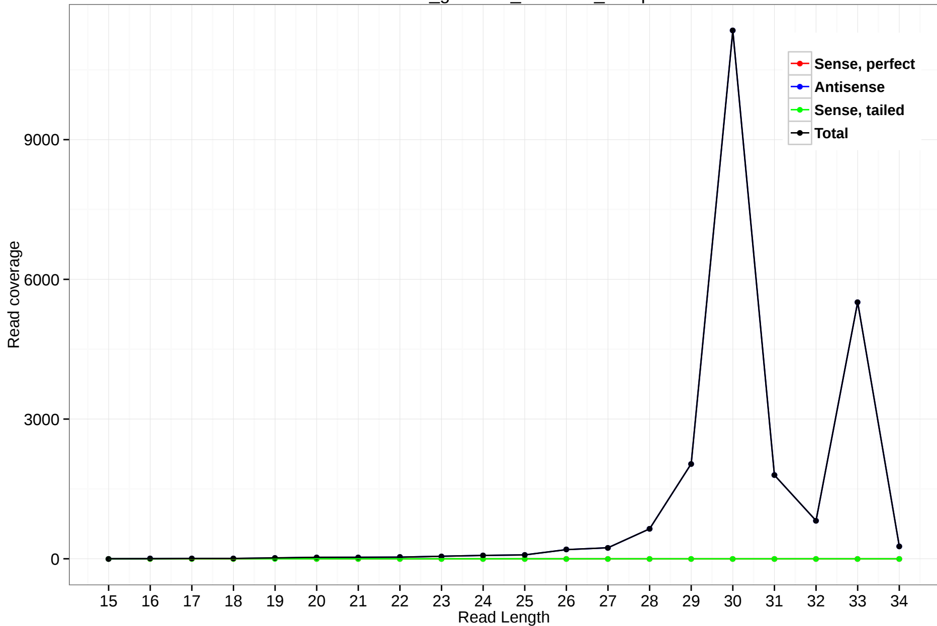
rheMac3_genscan_chr7.829_20.5p
