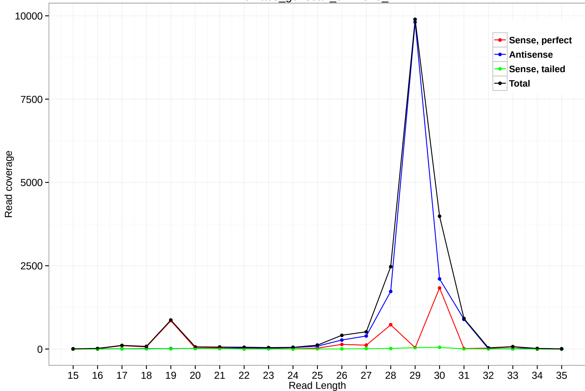
rheMac3_genscan_chr7.829_17
