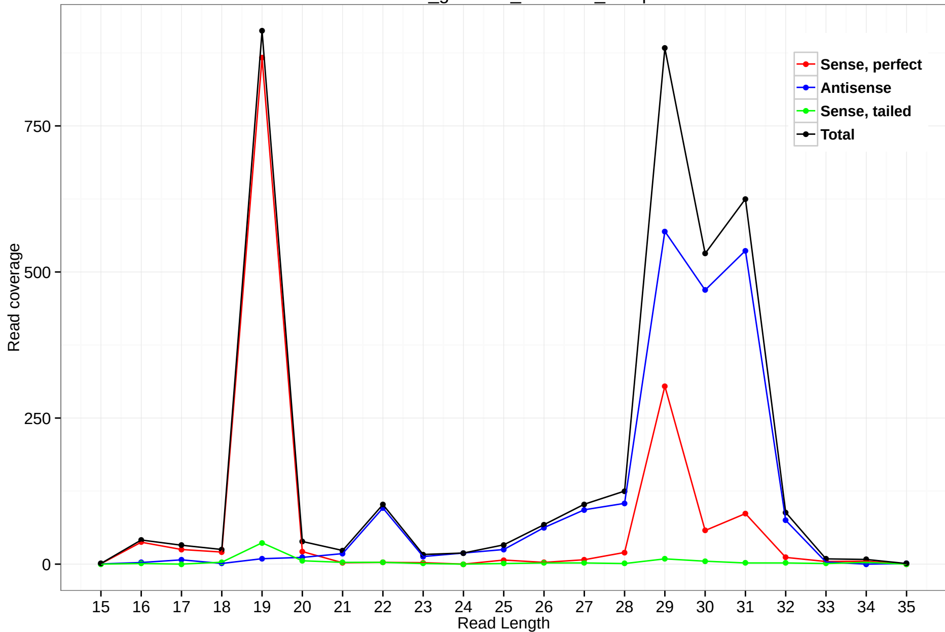
rheMac3_genscan_chr7.829_12.5p
