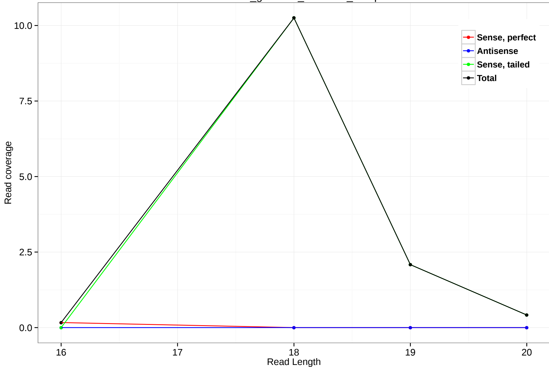
rheMac3_genscan_chr7.826_24.3p
