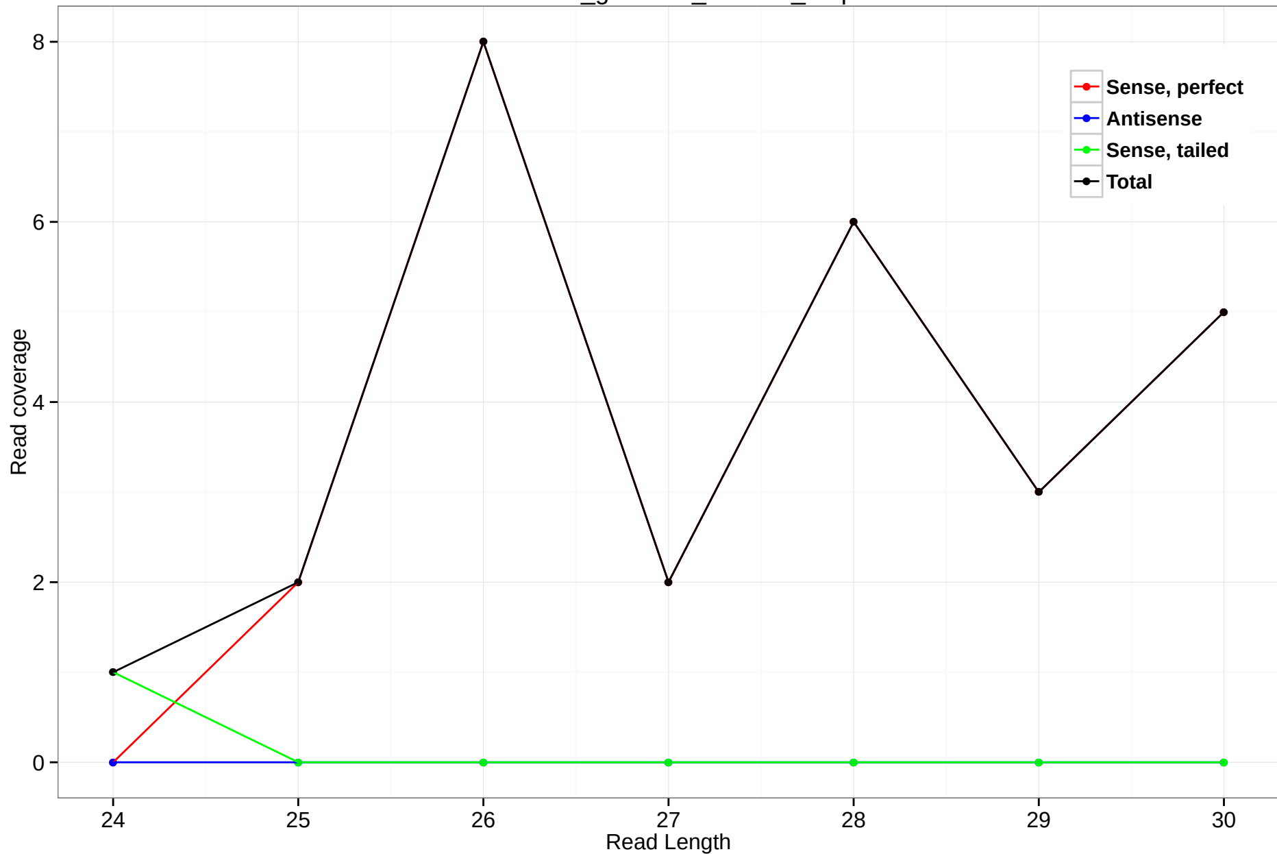
rheMac3_genscan_chr7.70_2.3p
