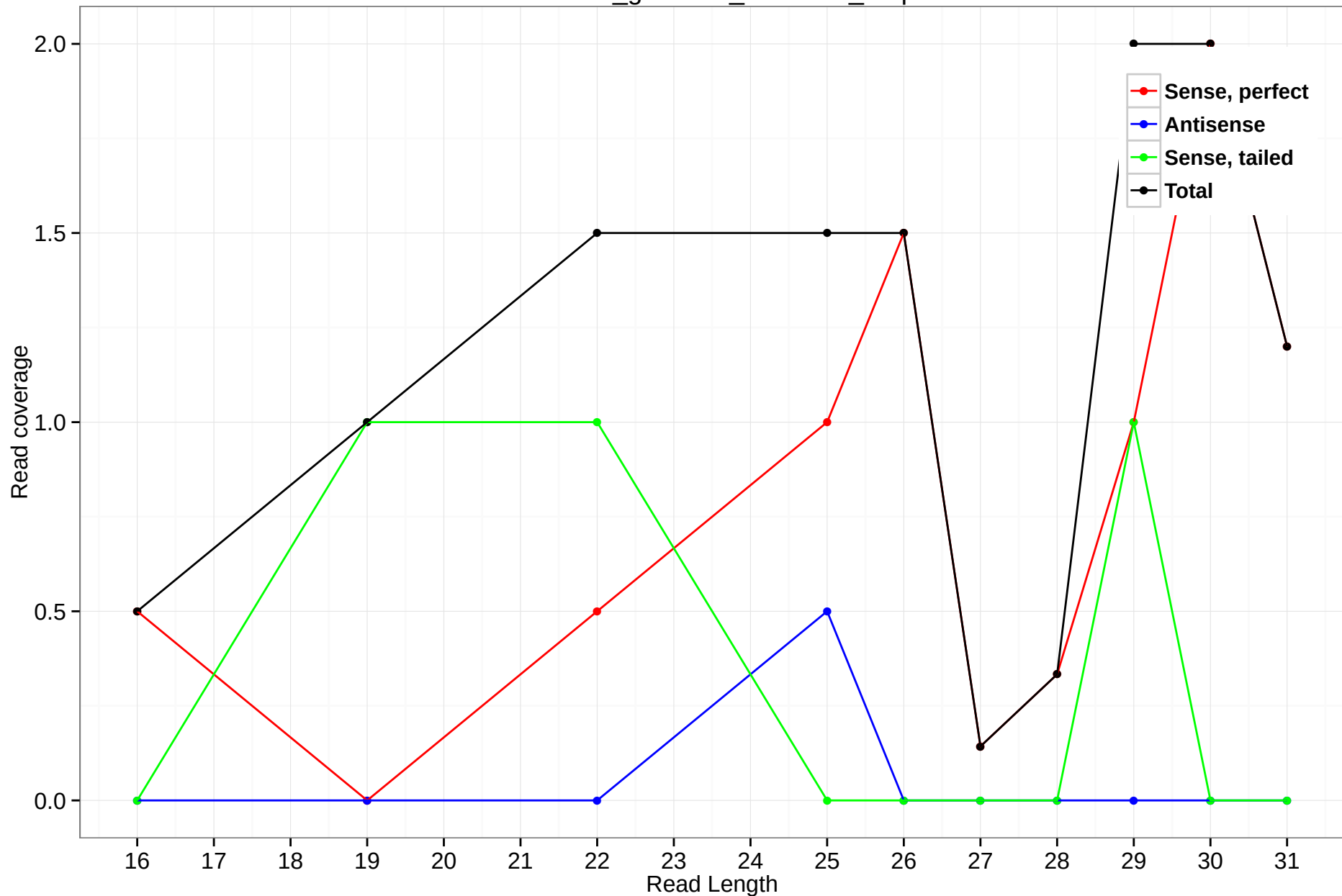
rheMac3_genscan_chr7.597_1.5p
