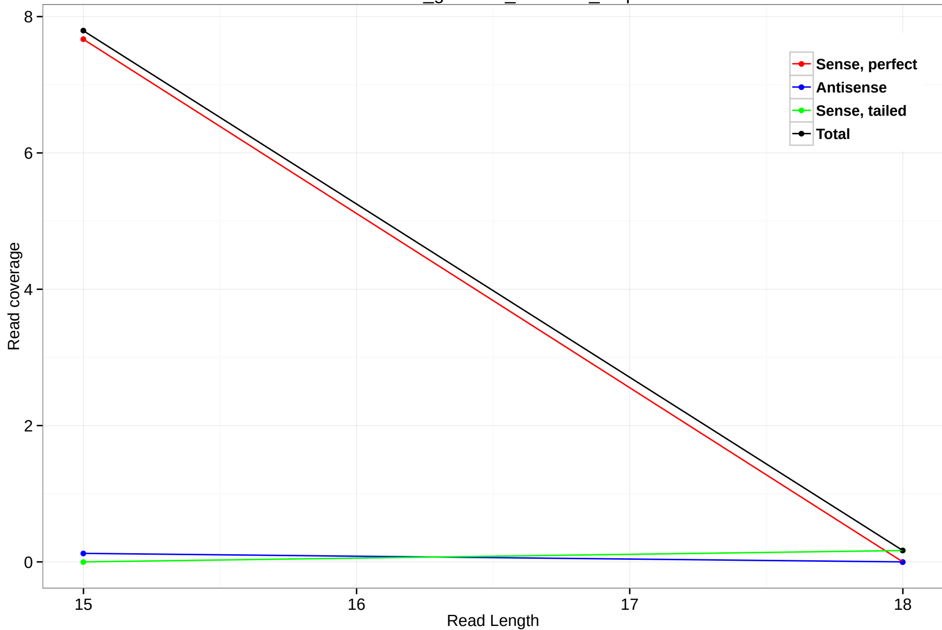
rheMac3_genscan_chr7.594_6.5p
