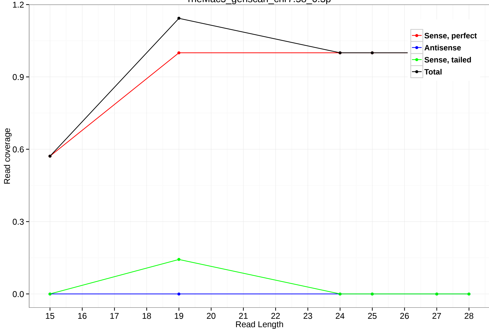
rheMac3_genscan_chr7.58_0.3p
