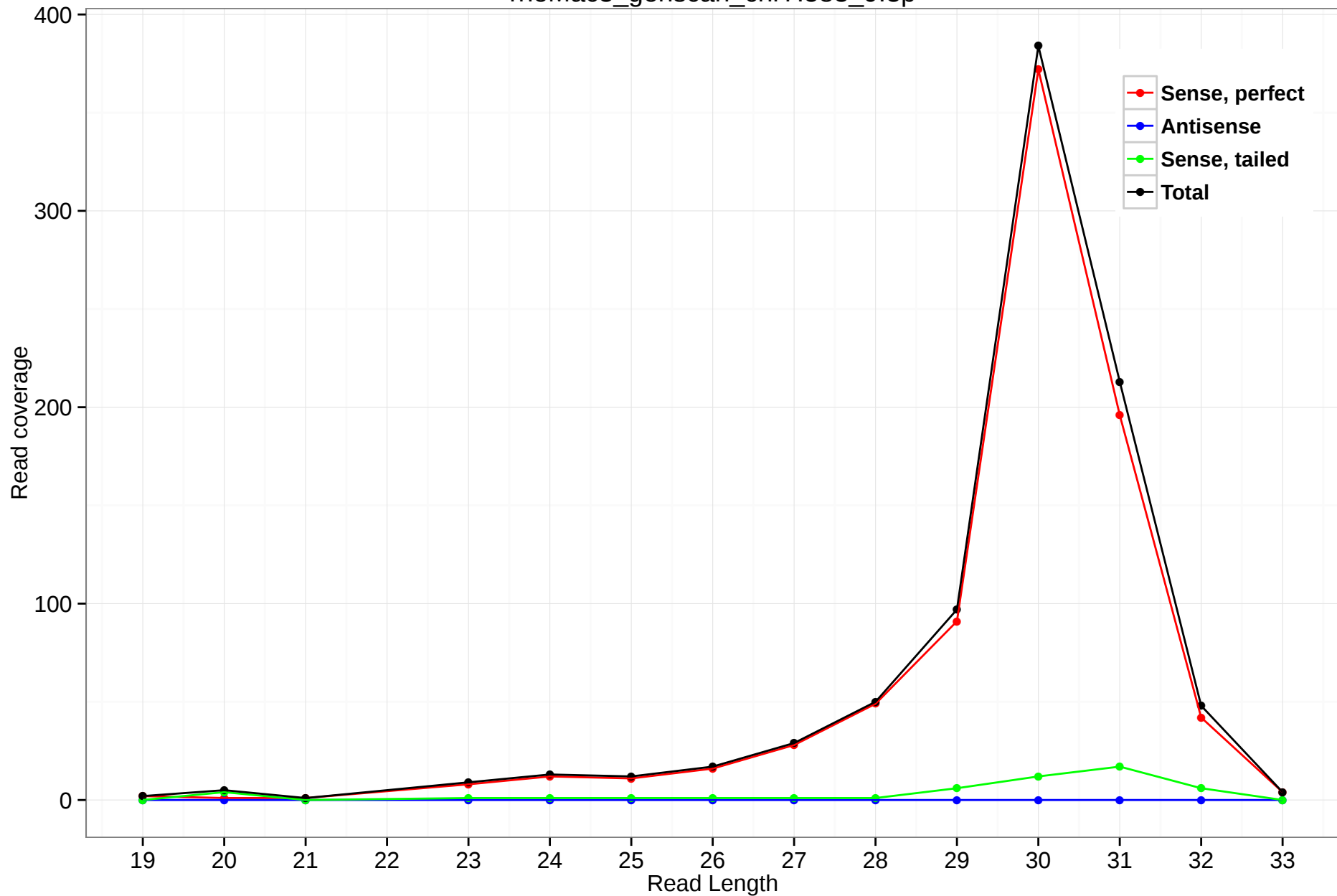
rheMac3_genscan_chr7.583_9.3p
