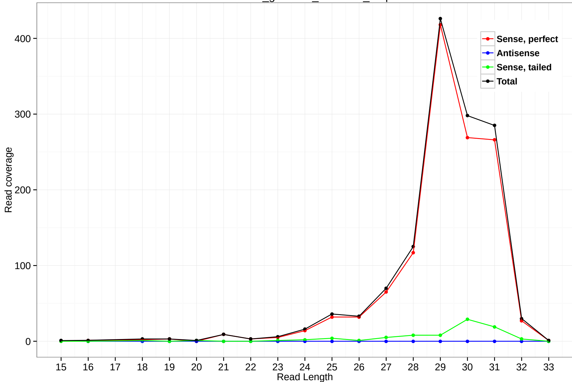
rheMac3_genscan_chr7.583_8.3p
