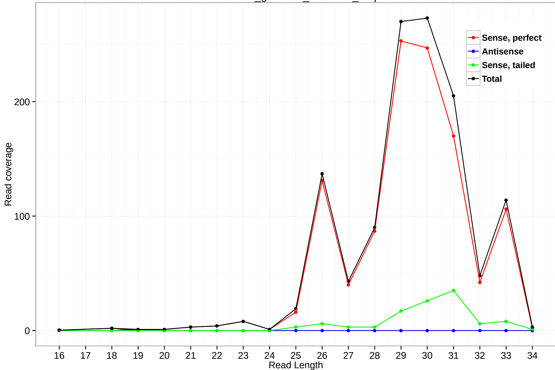
rheMac3_genscan_chr7.583_6.3p
