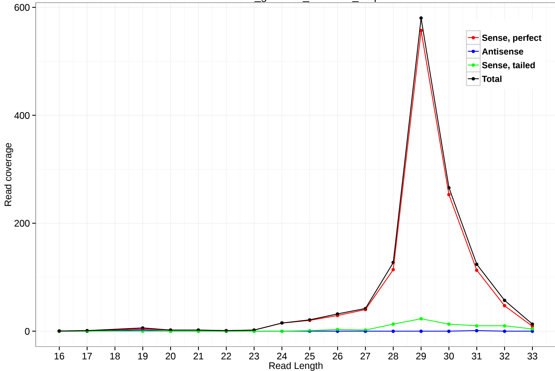
rheMac3_genscan_chr7.583_4.5p
