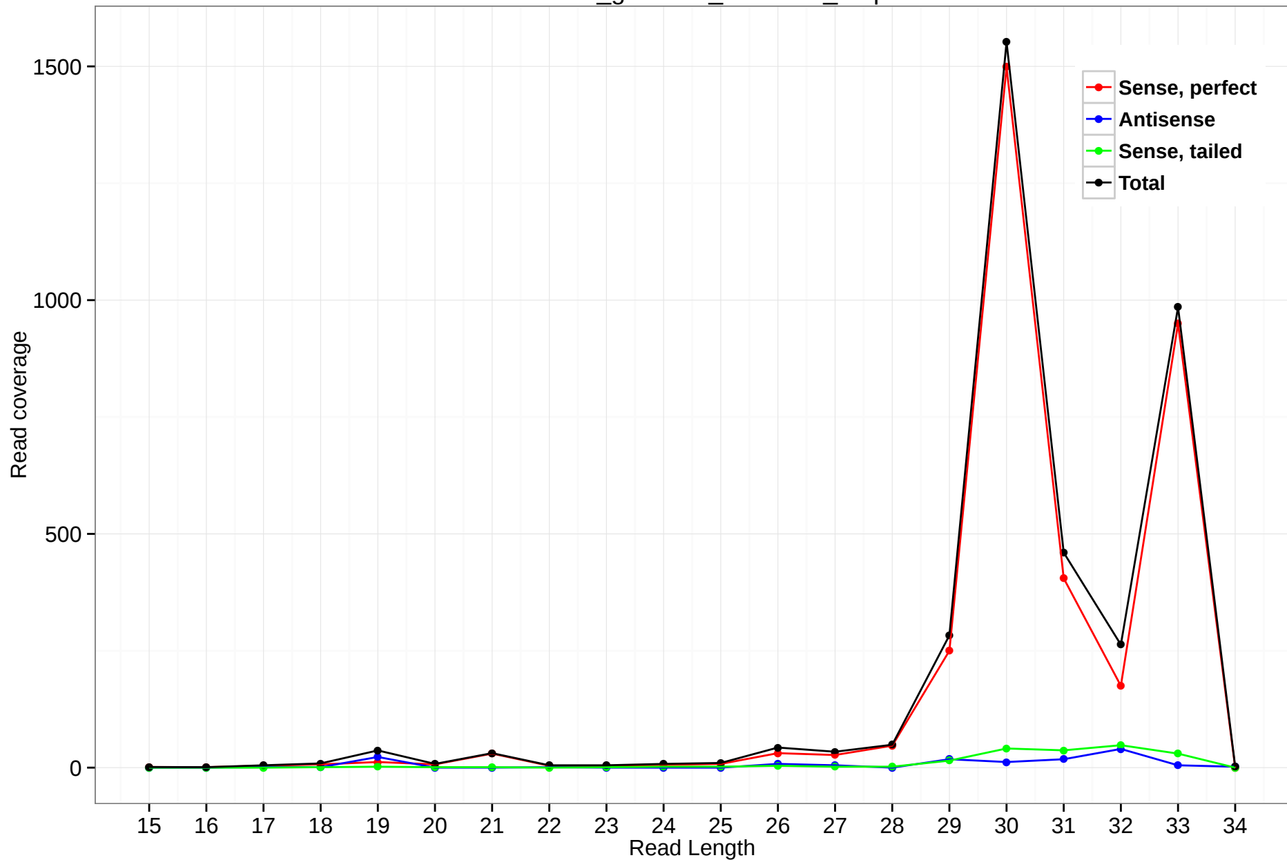
rheMac3_genscan_chr7.583_3.3p
