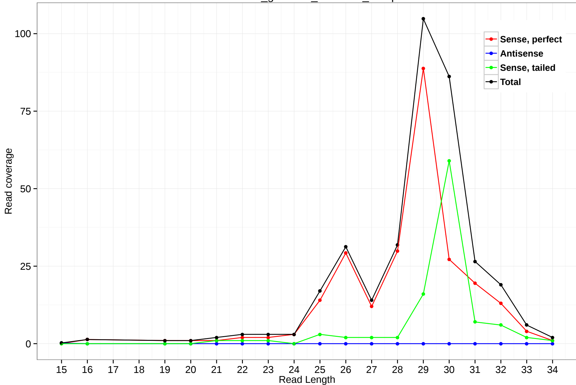
rheMac3_genscan_chr7.583_10.5p
