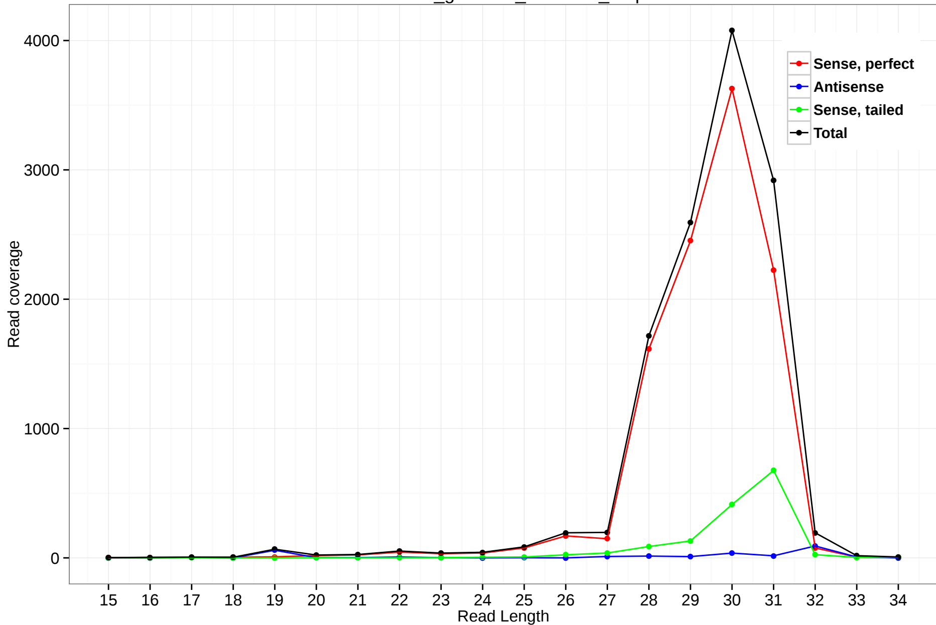
rheMac3_genscan_chr7.583_1.5p
