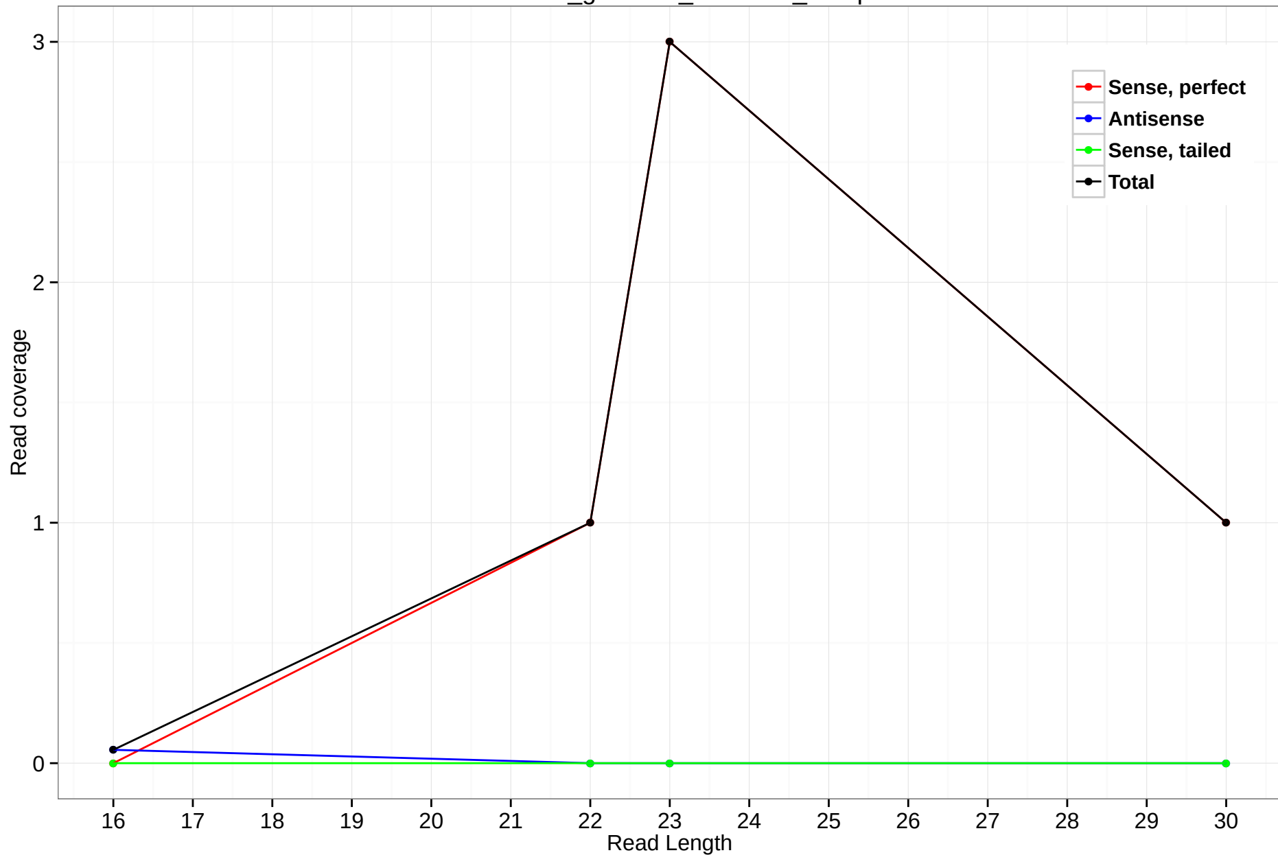
rheMac3_genscan_chr7.549_23.5p
