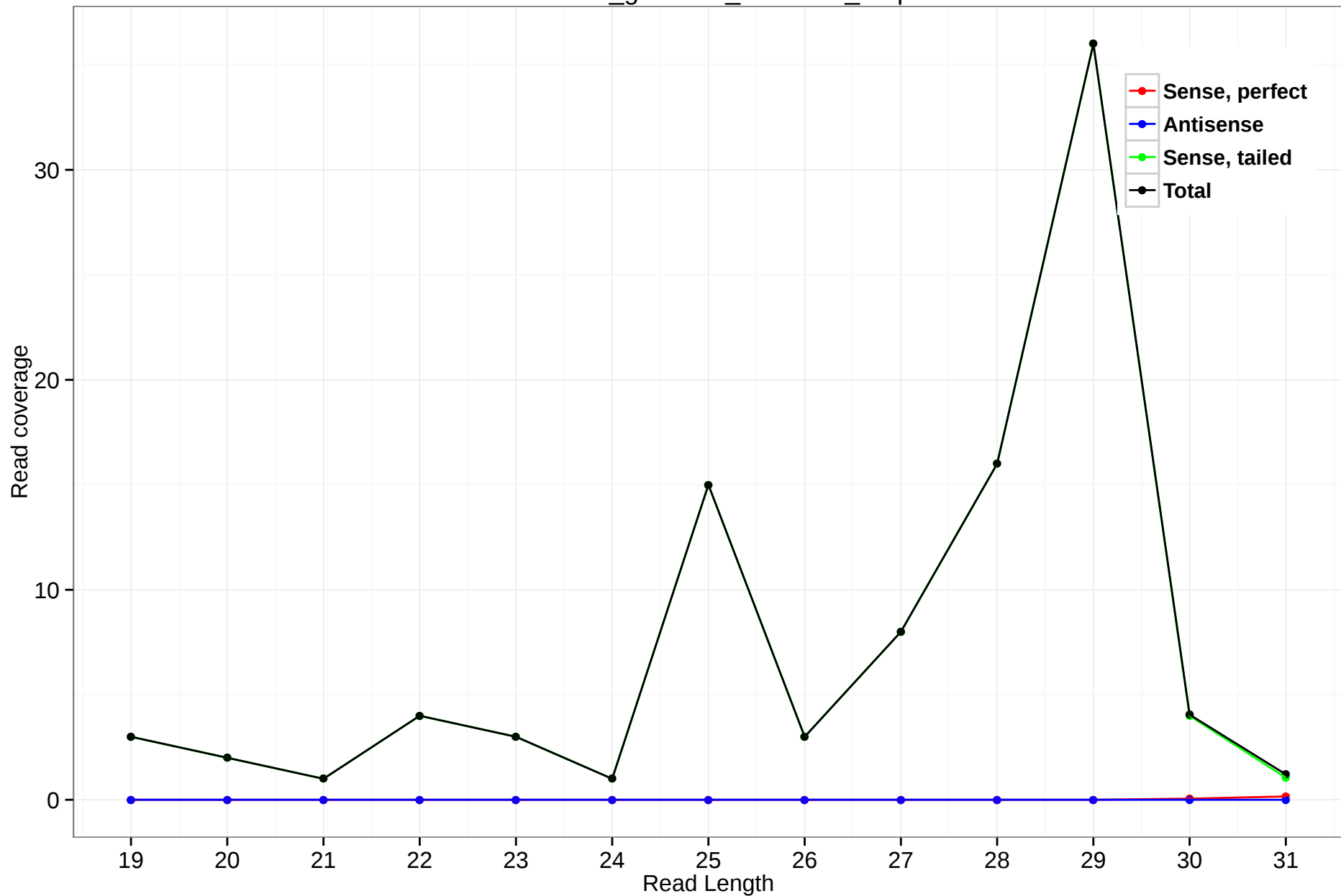
rheMac3_genscan_chr7.468_2.3p
