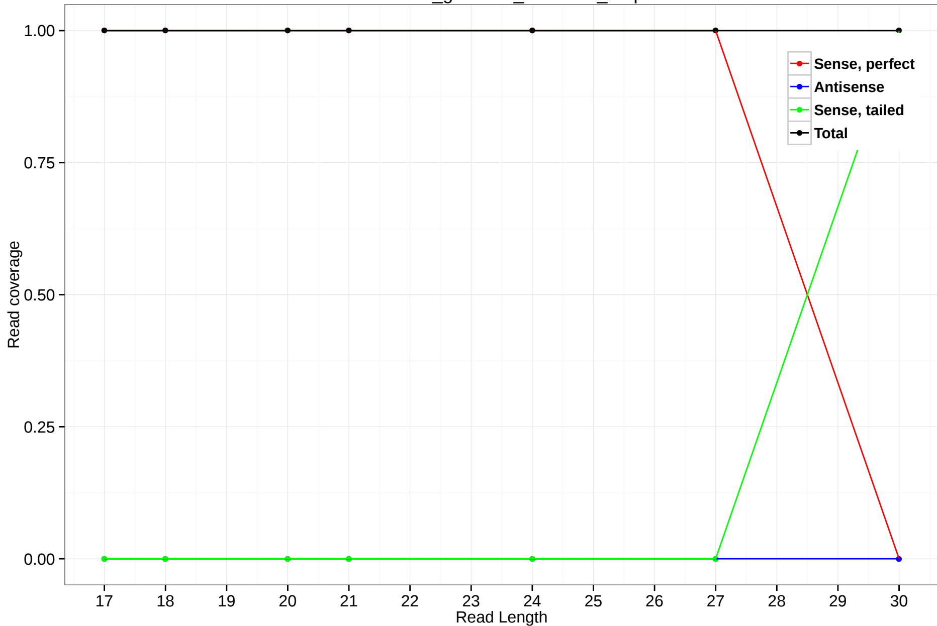
rheMac3_genscan_chr7.453_2.5p
