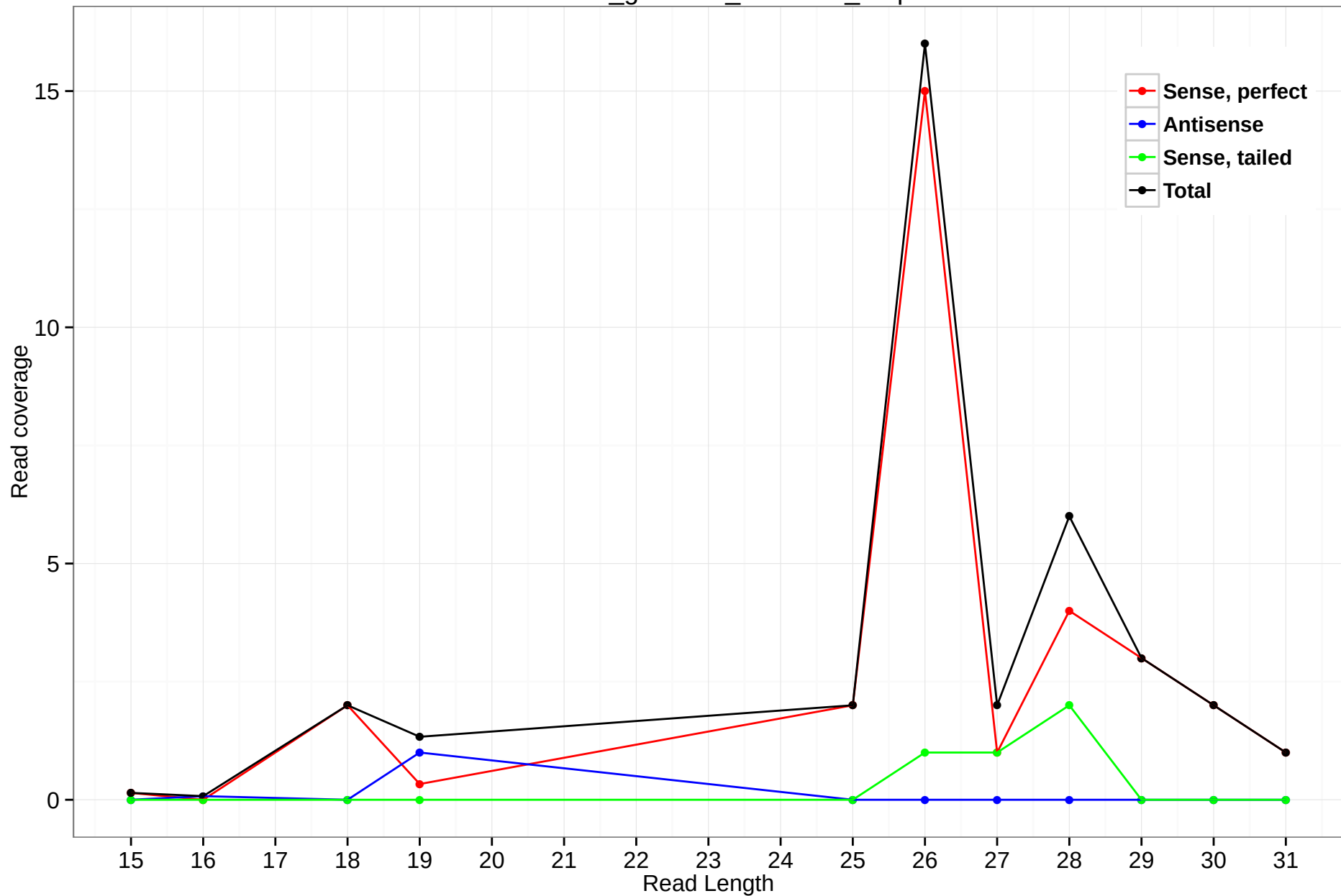
rheMac3_genscan_chr7.415_5.5p
