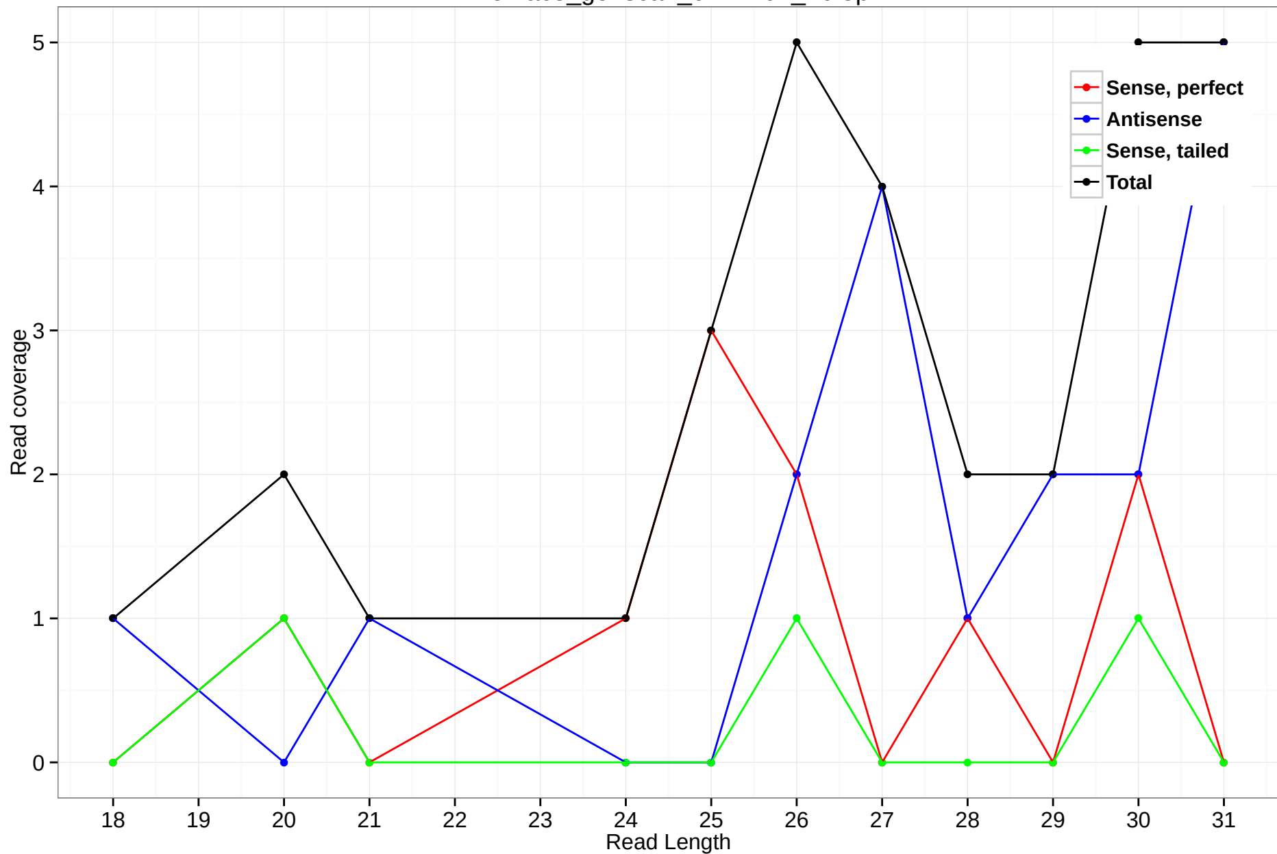
rheMac3_genscan_chr7.407_16.5p
