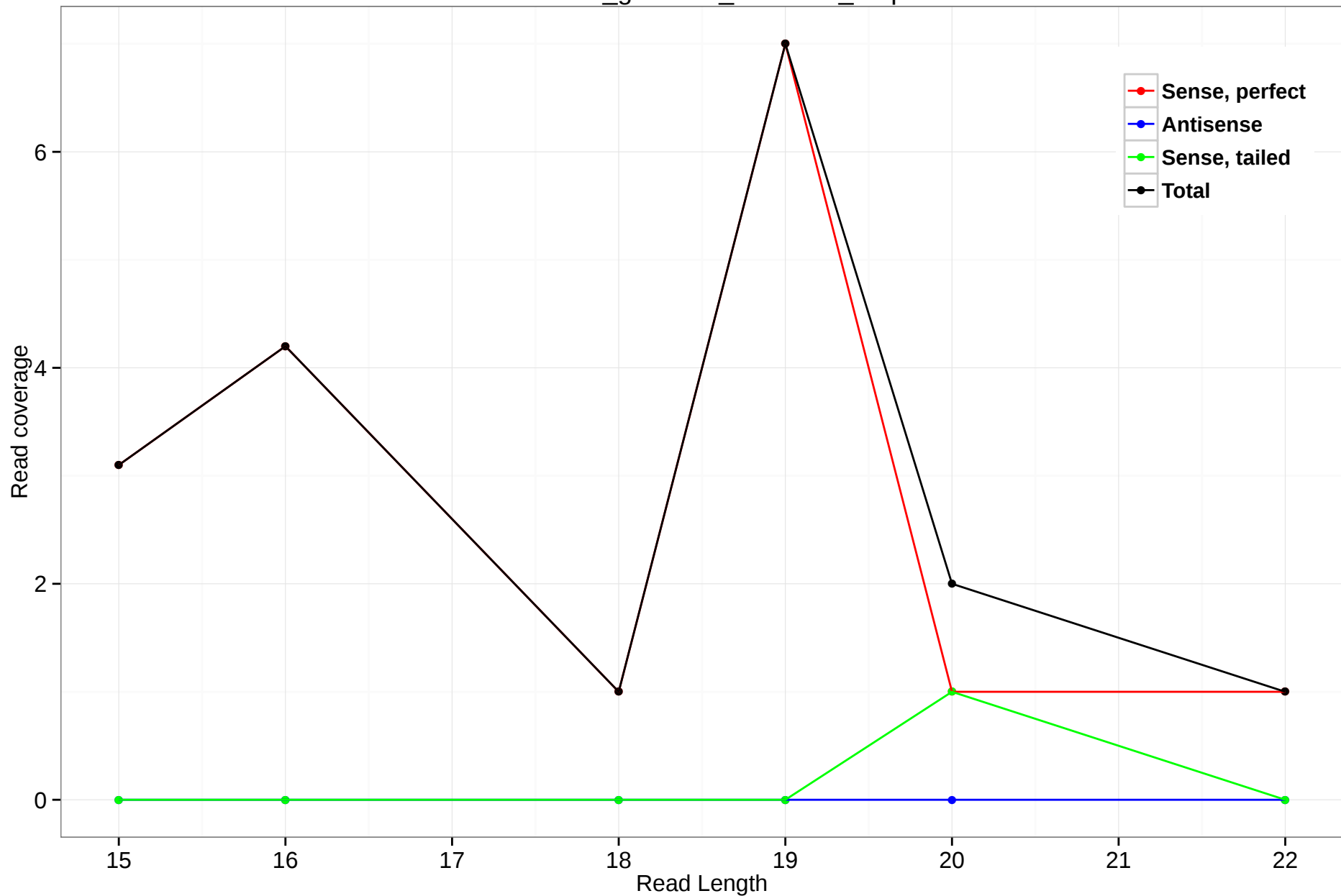
rheMac3_genscan_chr7.398_2.5p
