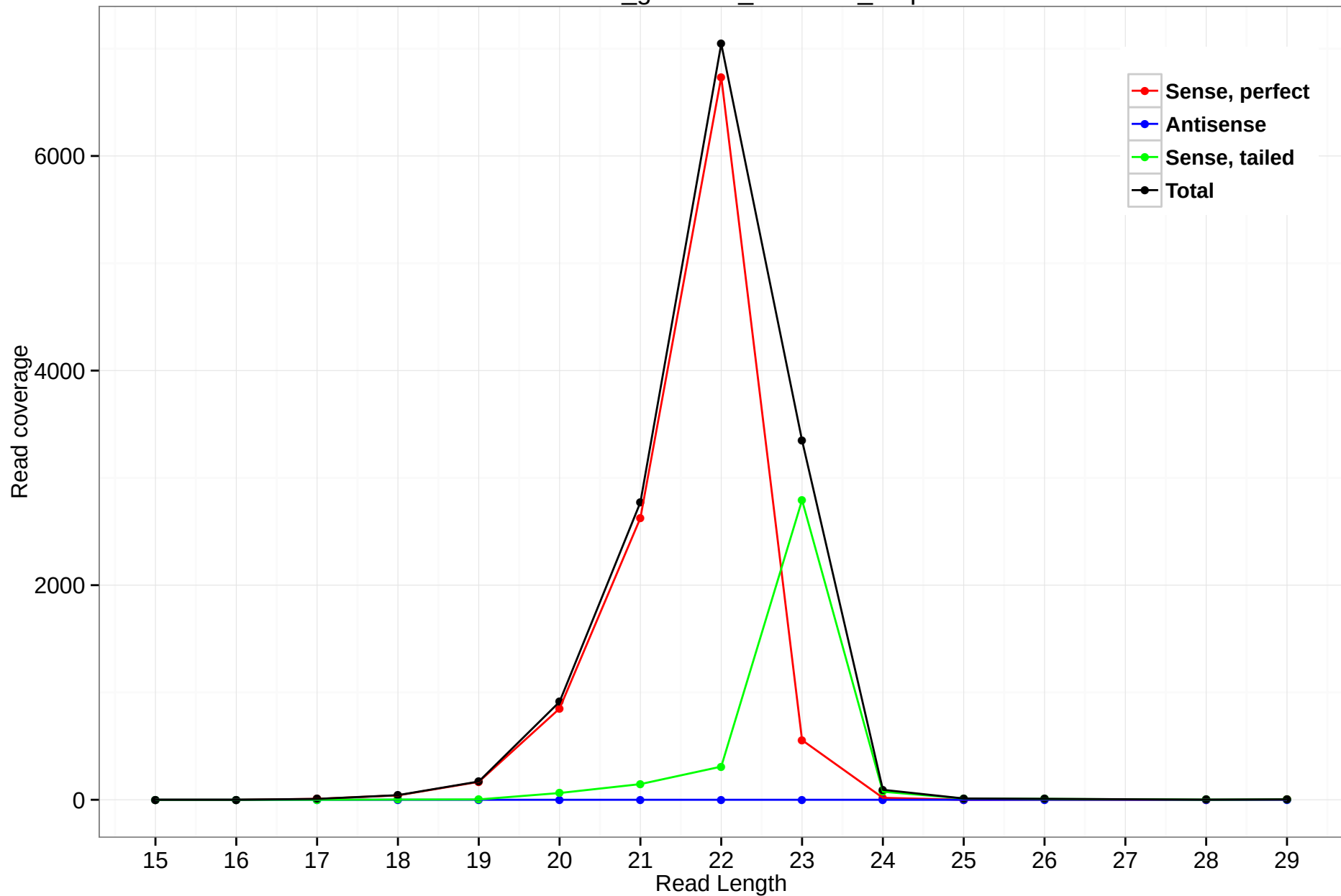
rheMac3_genscan_chr7.374_1.5p
