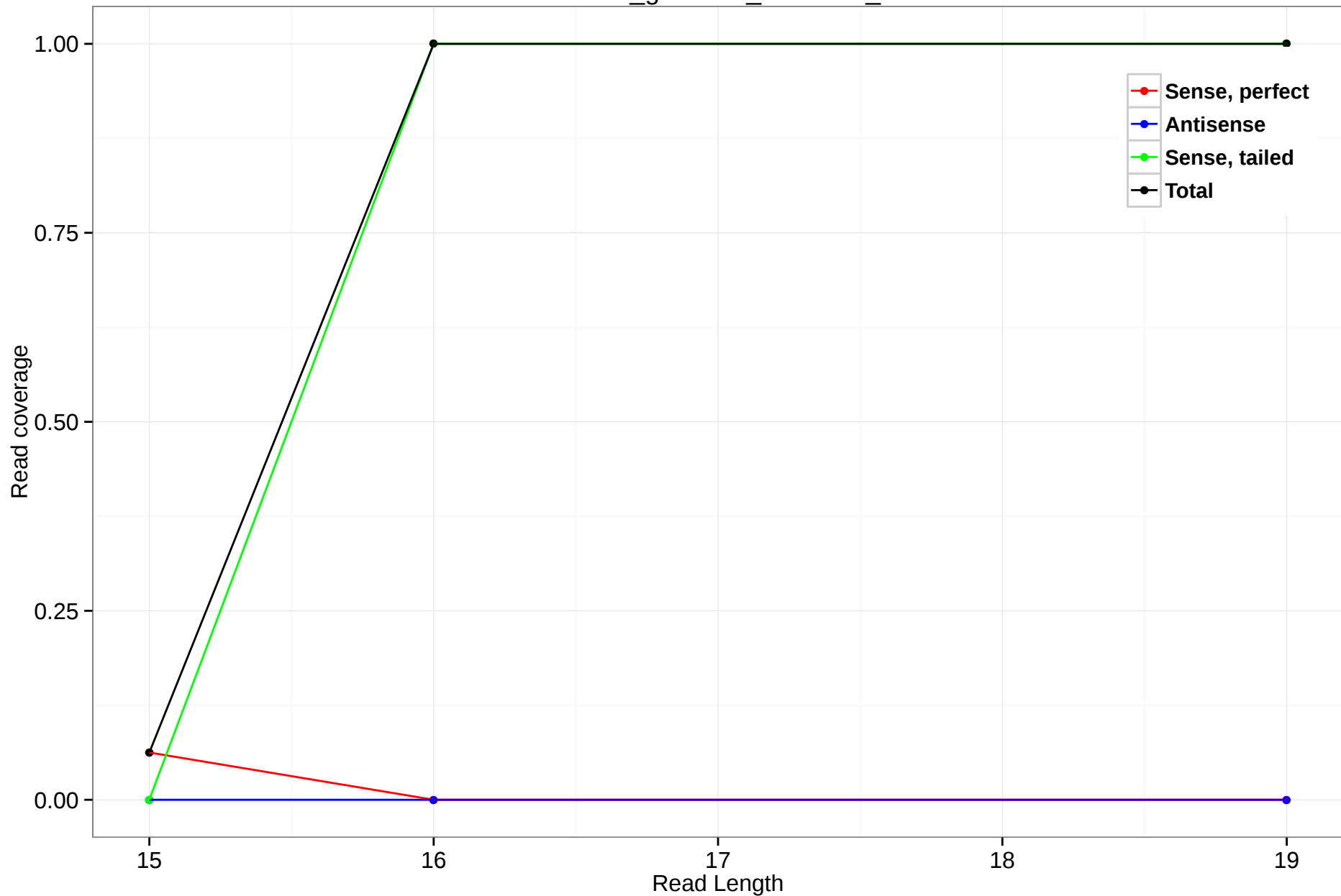
rheMac3_genscan_chr7.371_41
