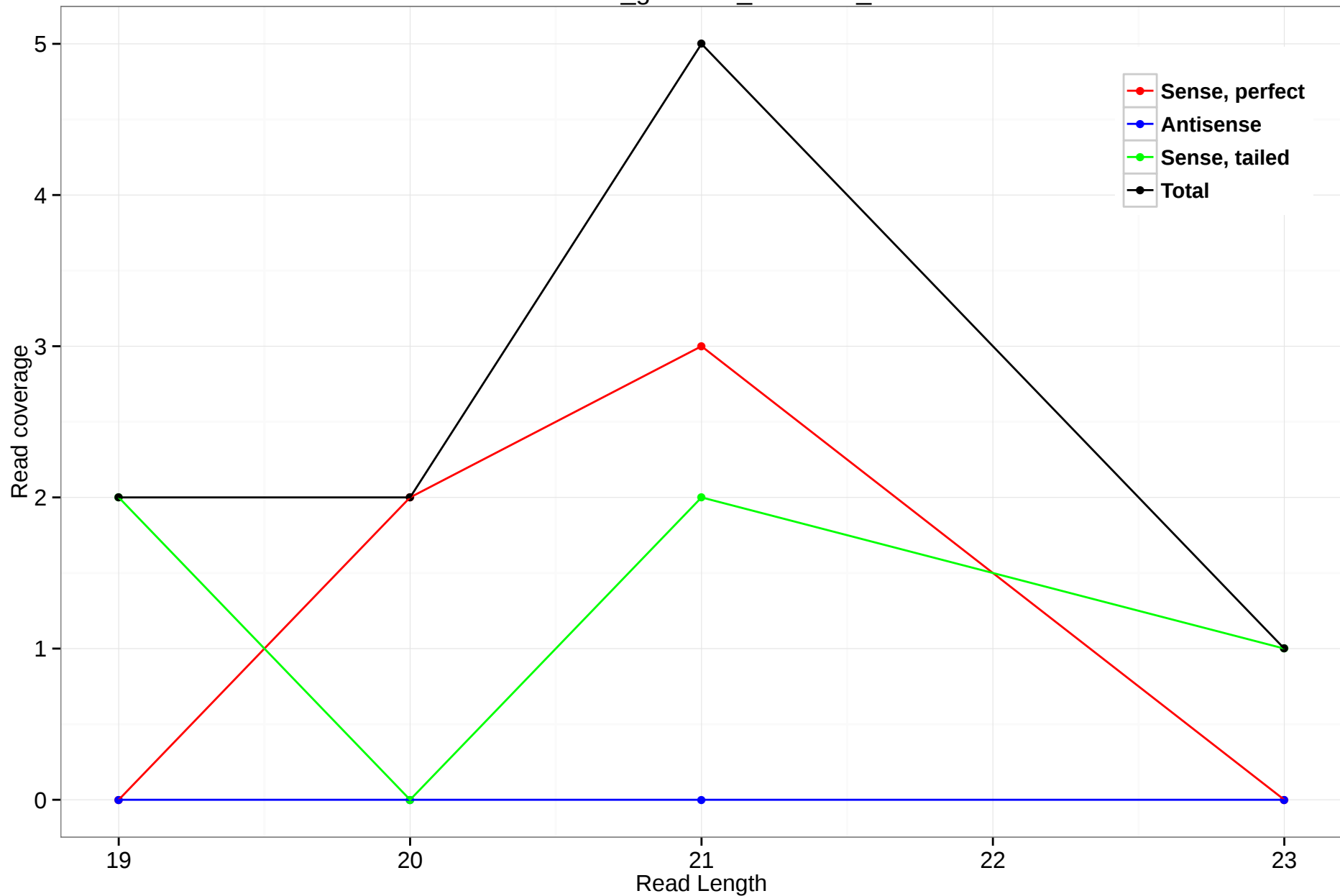
rheMac3_genscan_chr7.369_5
