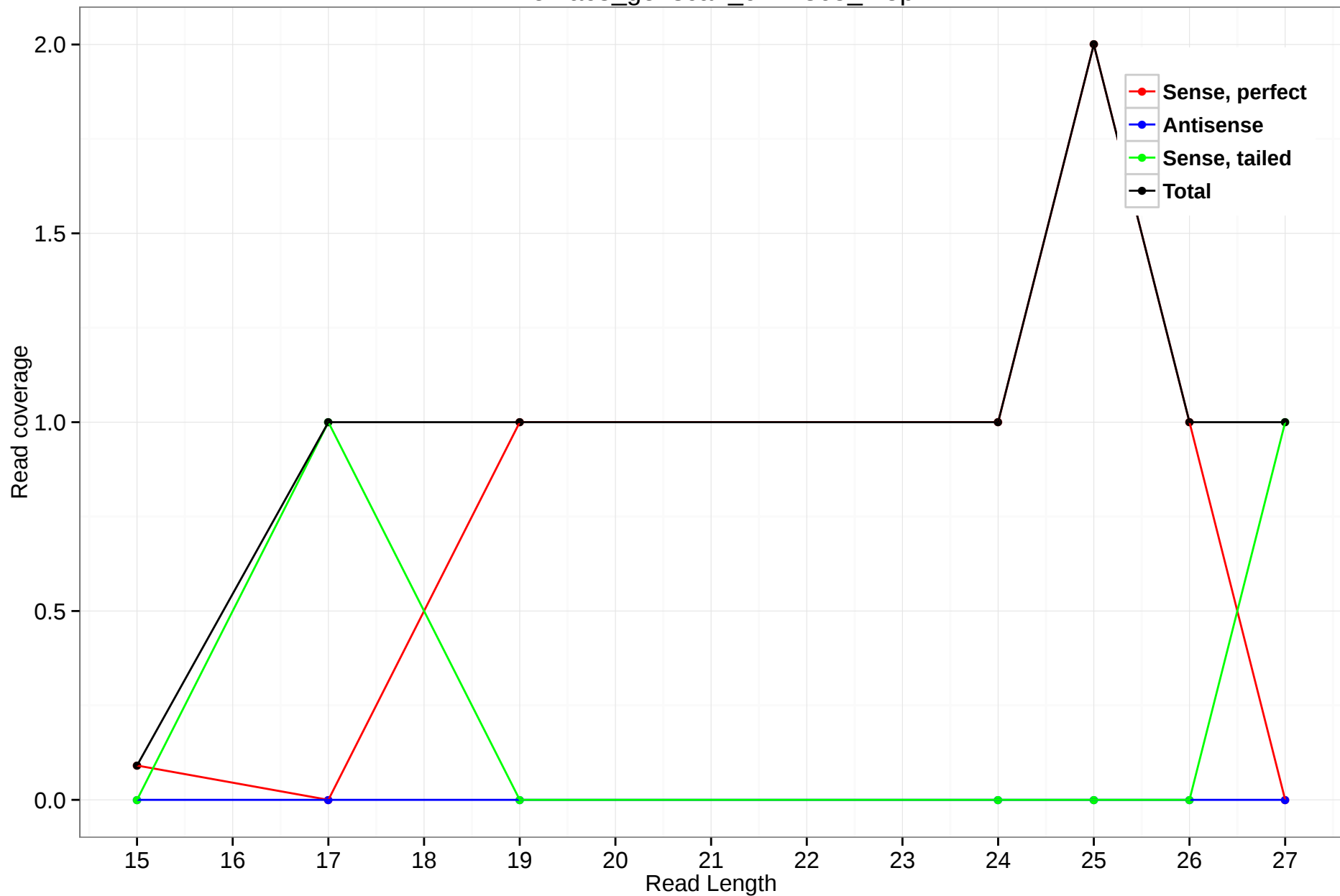
rheMac3_genscan_chr7.365_2.5p
