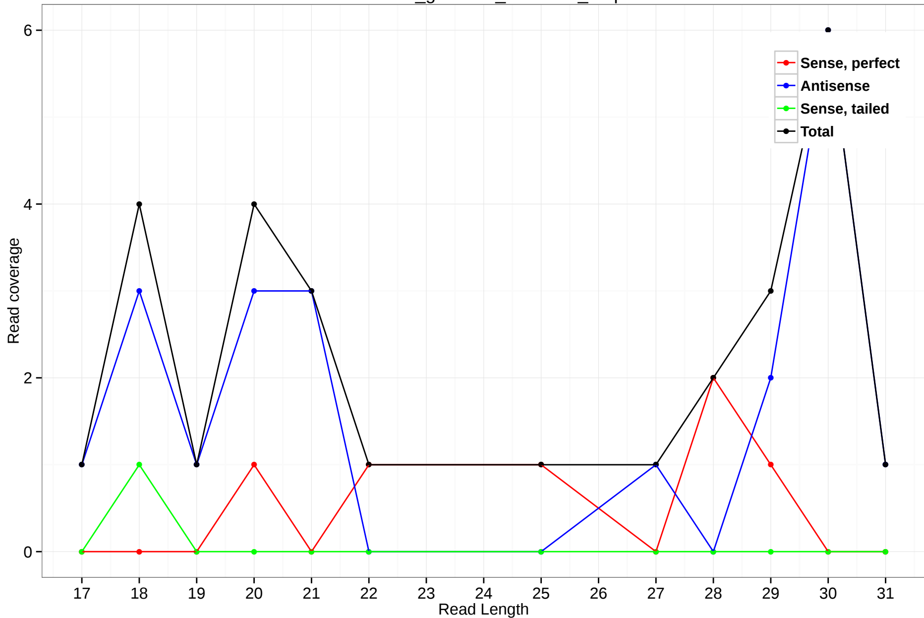
rheMac3_genscan_chr7.348_1.5p
