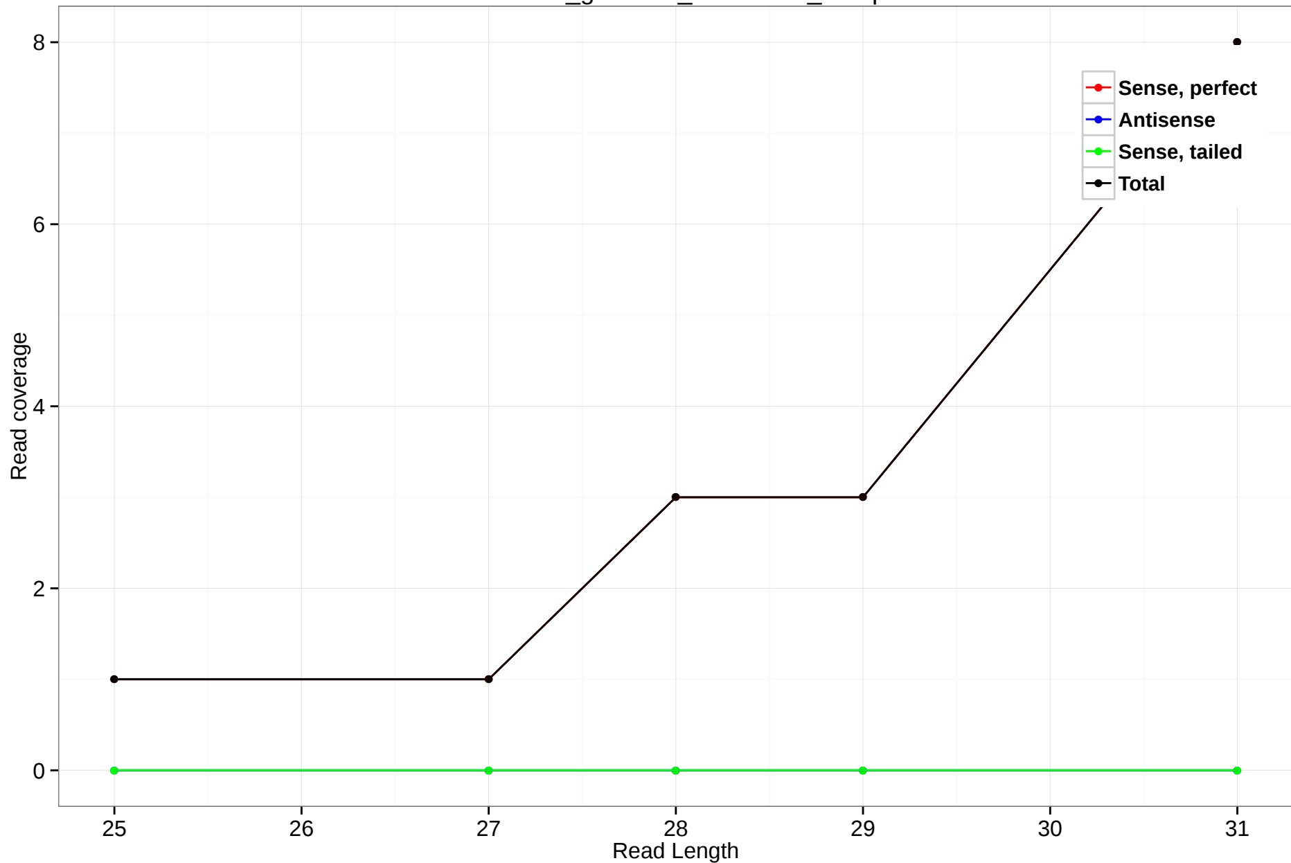
rheMac3_genscan_chr7.3323_20.3p
