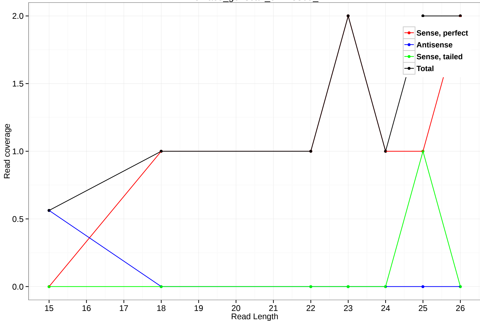
rheMac3_genscan_chr7.3309_4
