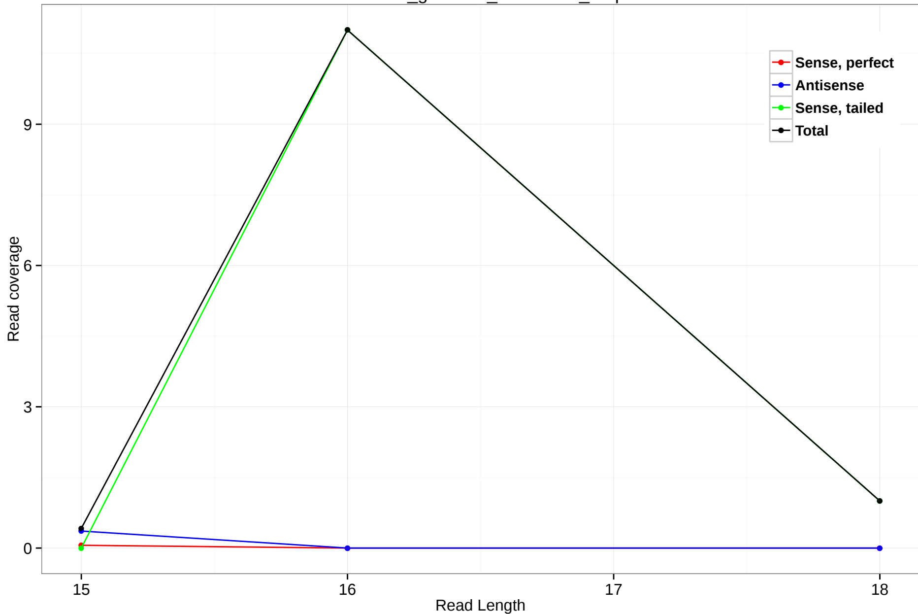
rheMac3_genscan_chr7.3301_5.5p
