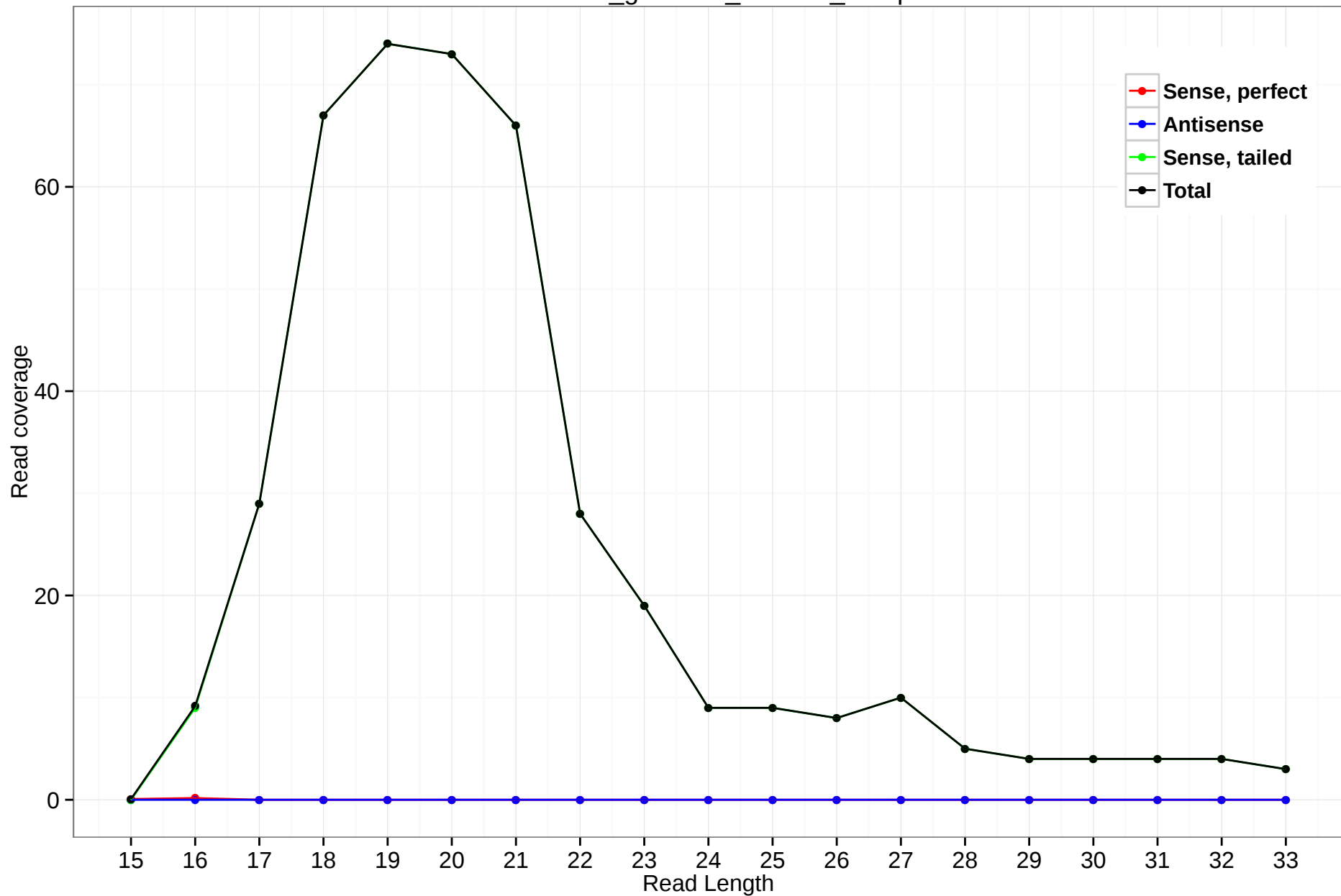
rheMac3_genscan_chr7.32_56.3p
