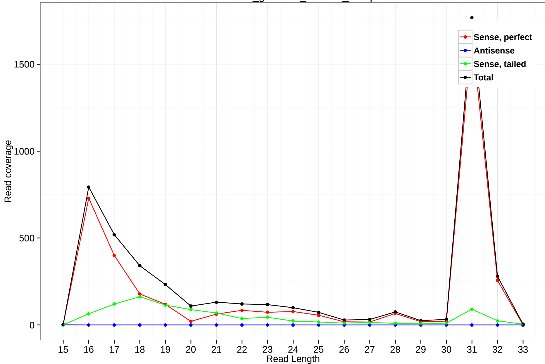
rheMac3_genscan_chr7.32_52.5p
