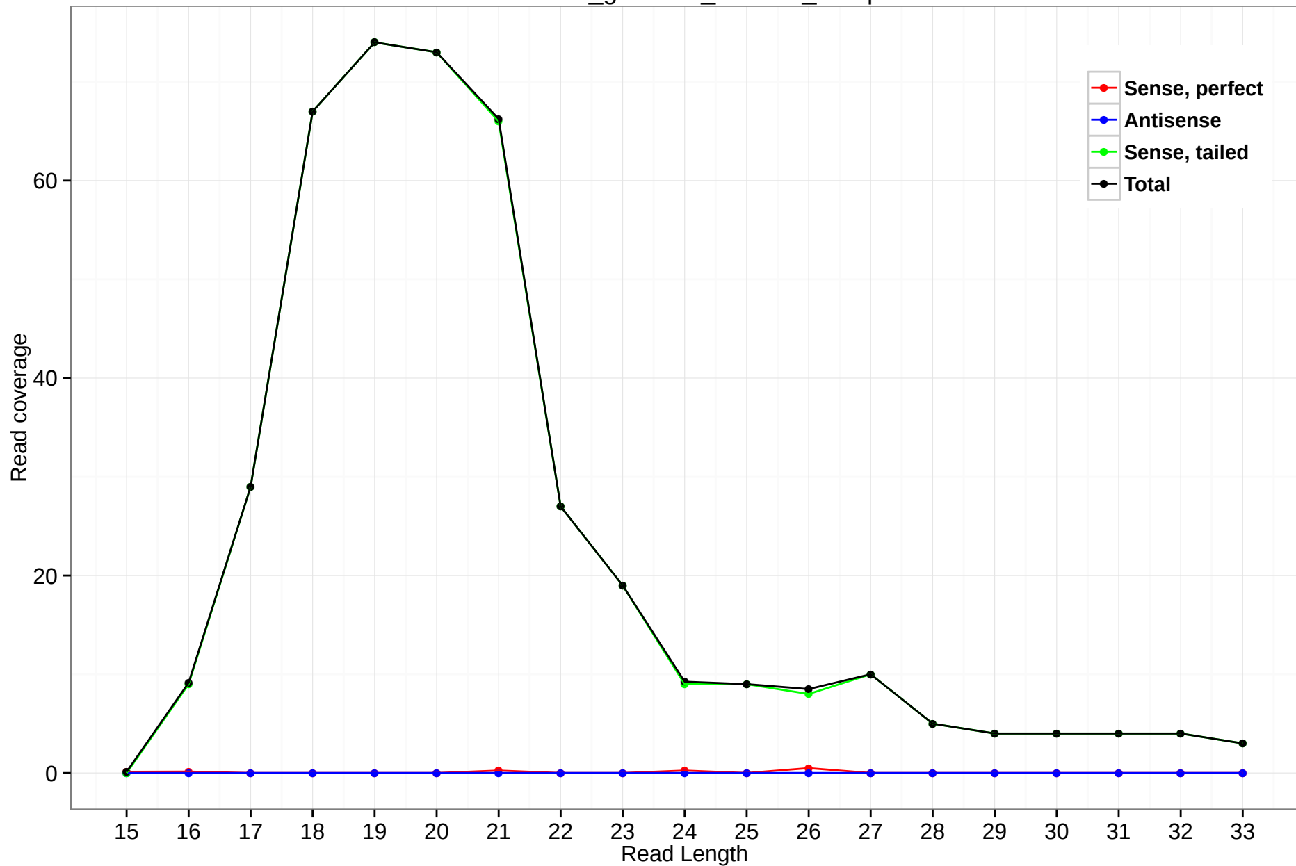
rheMac3_genscan_chr7.32_48.3p
