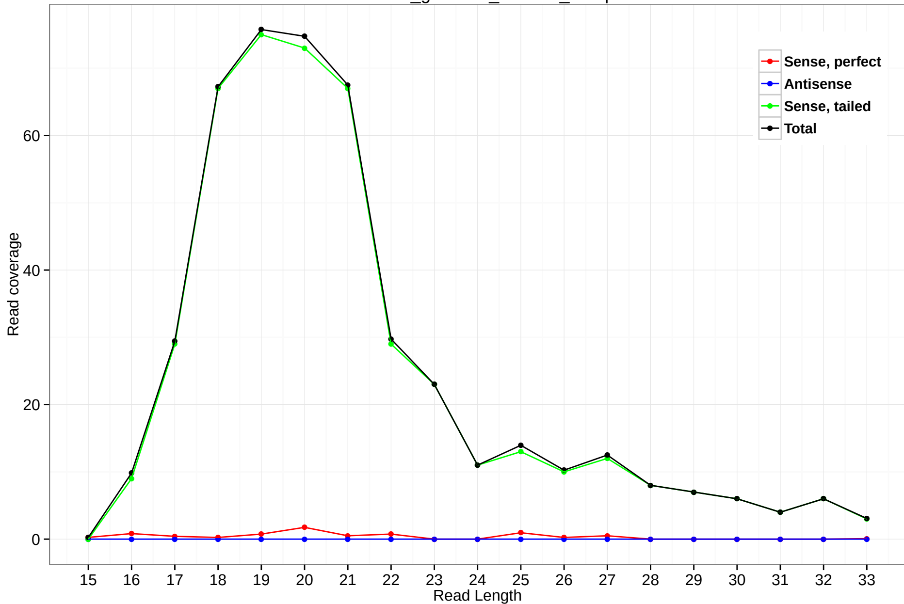
rheMac3_genscan_chr7.32_44.3p
