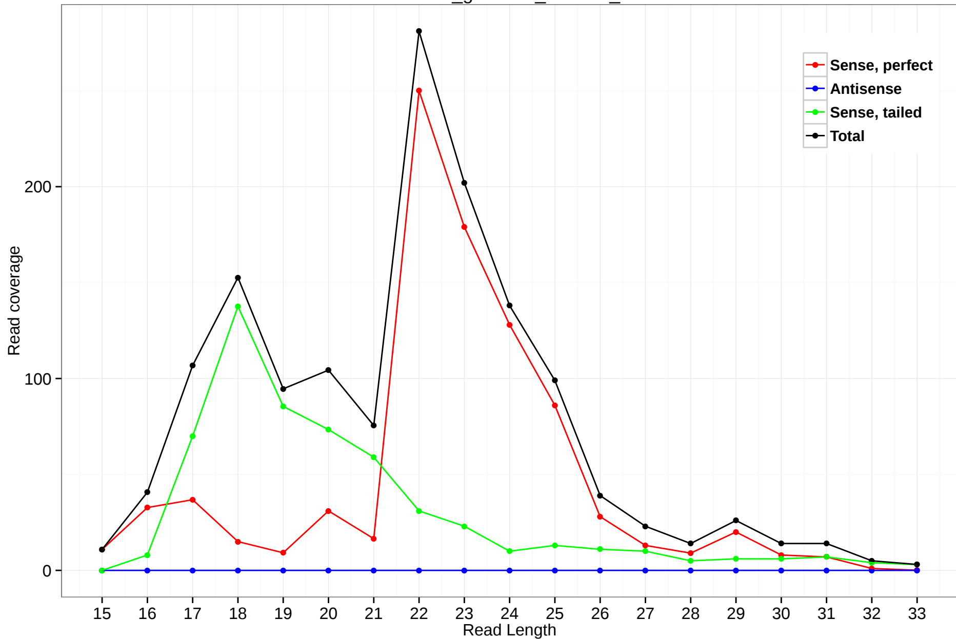
rheMac3_genscan_chr7.32_40
