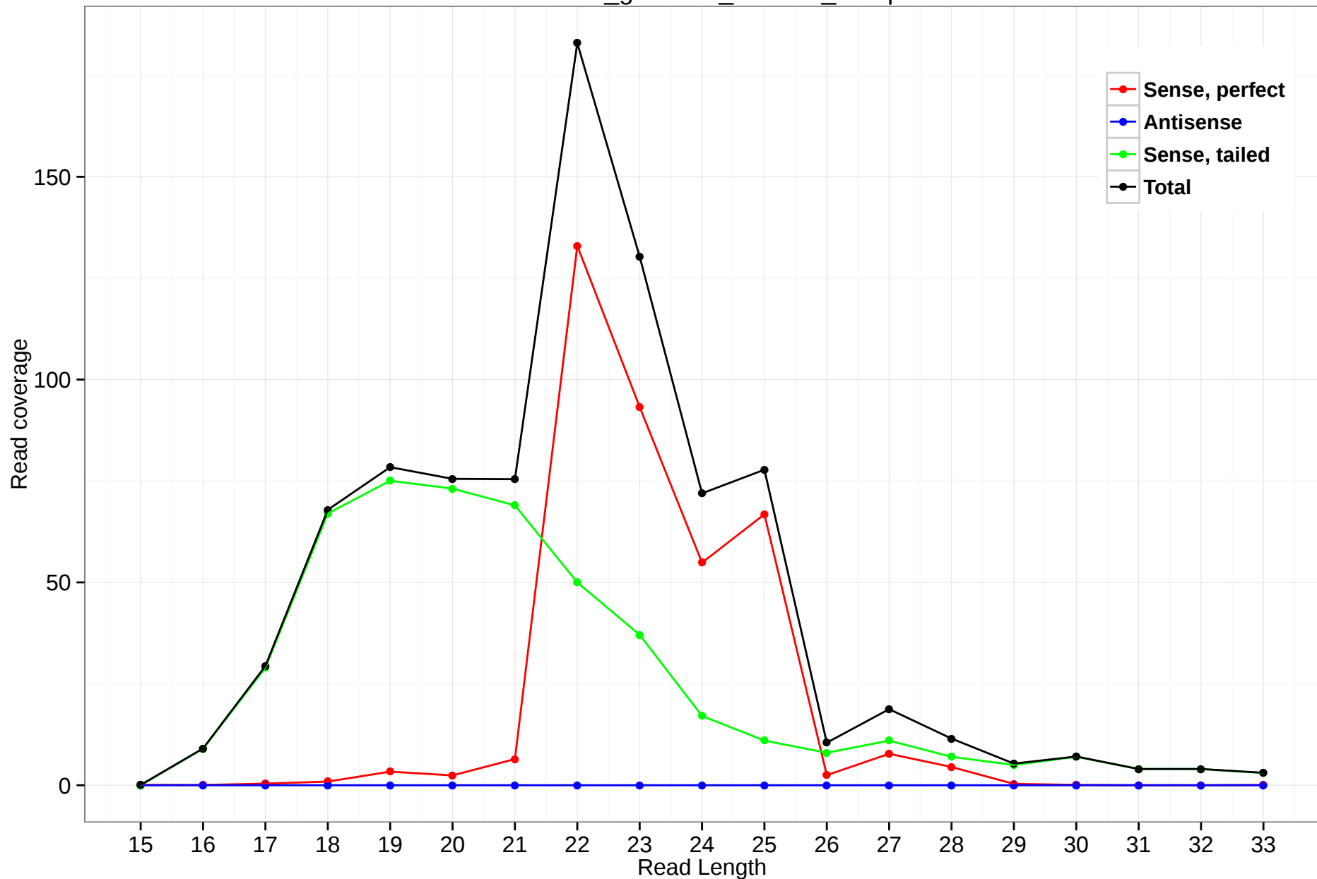
rheMac3_genscan_chr7.32_32.3p
