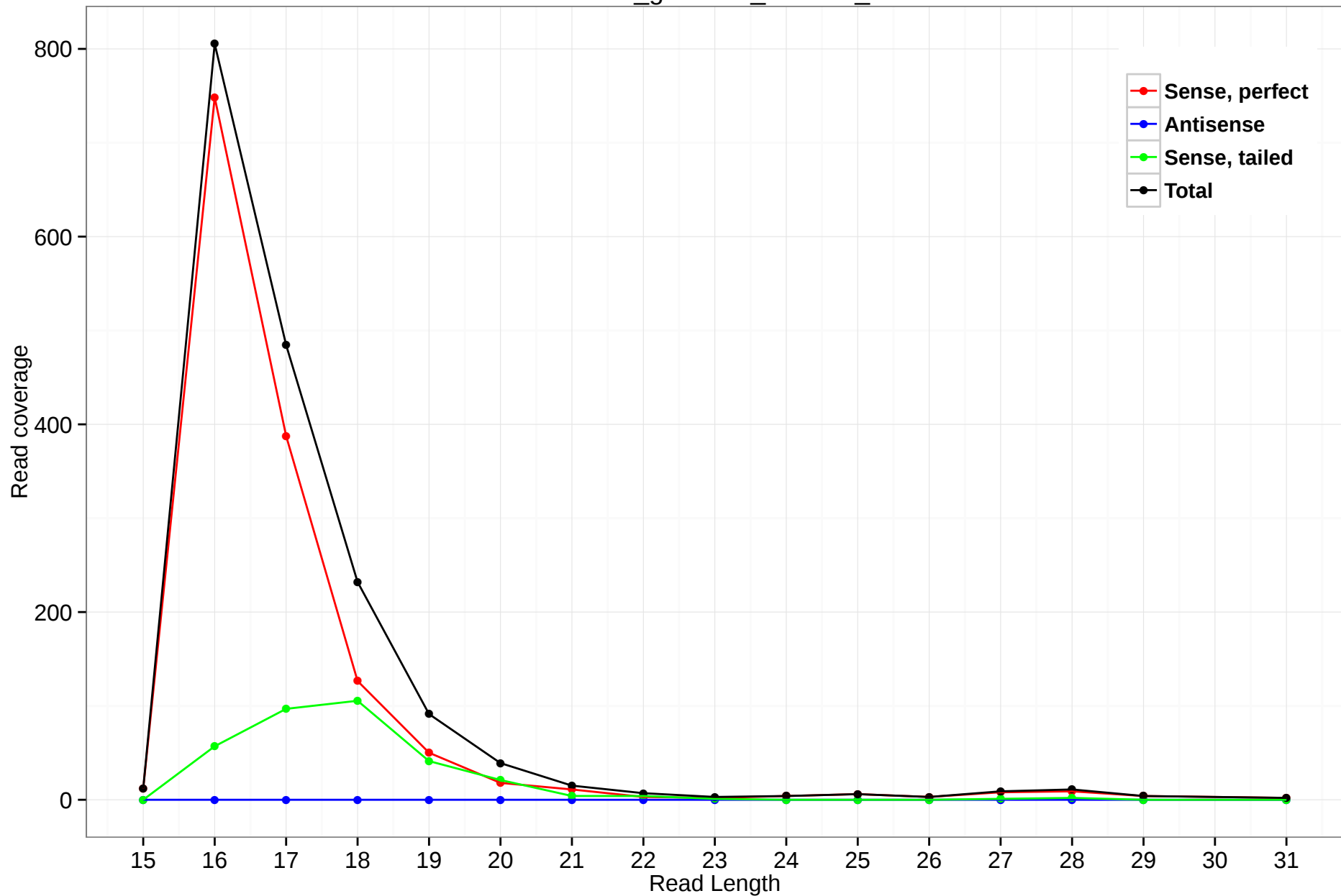
rheMac3_genscan_chr7.32_31
