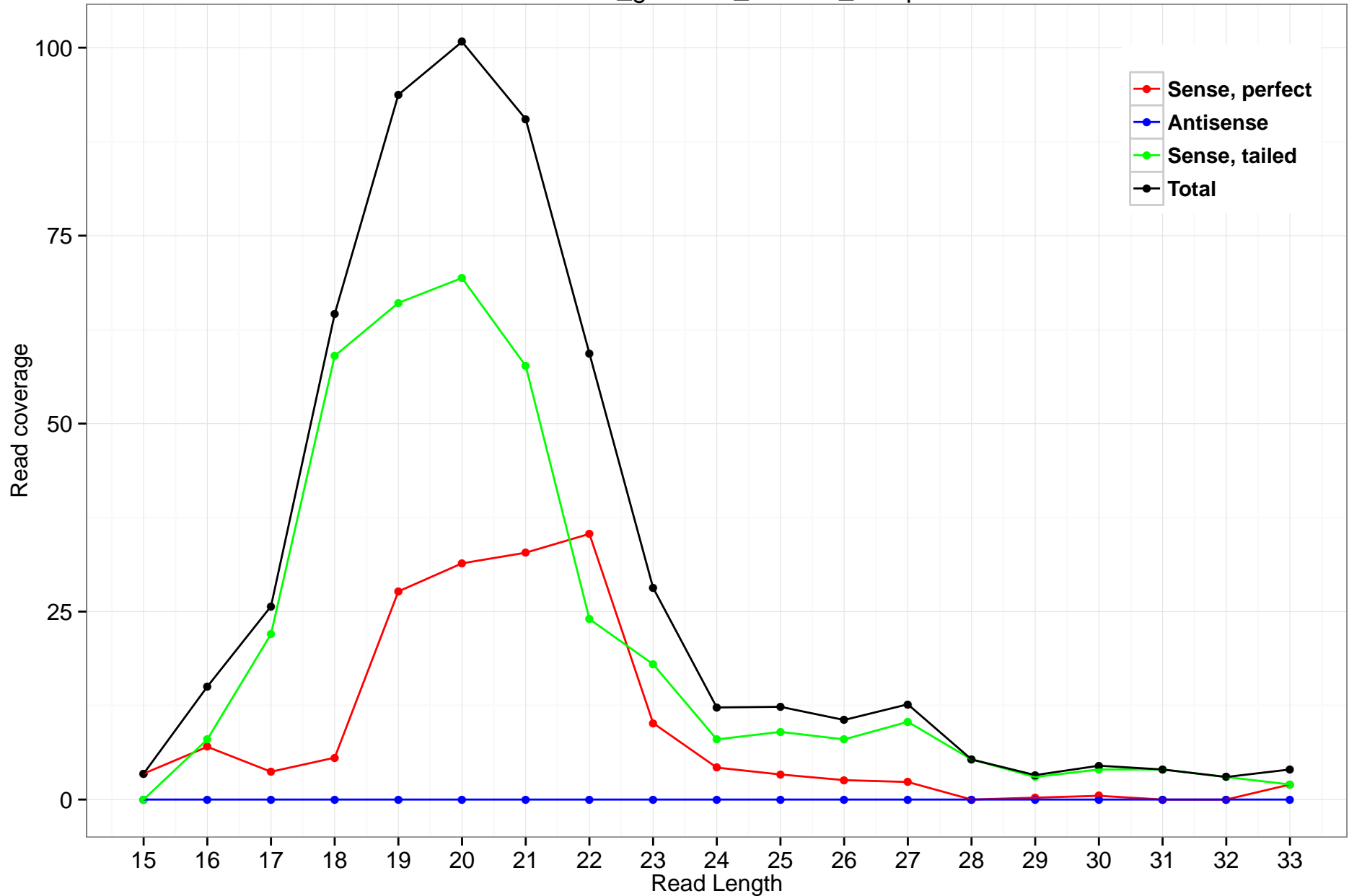
rheMac3_genscan_chr7.32_17.3p
