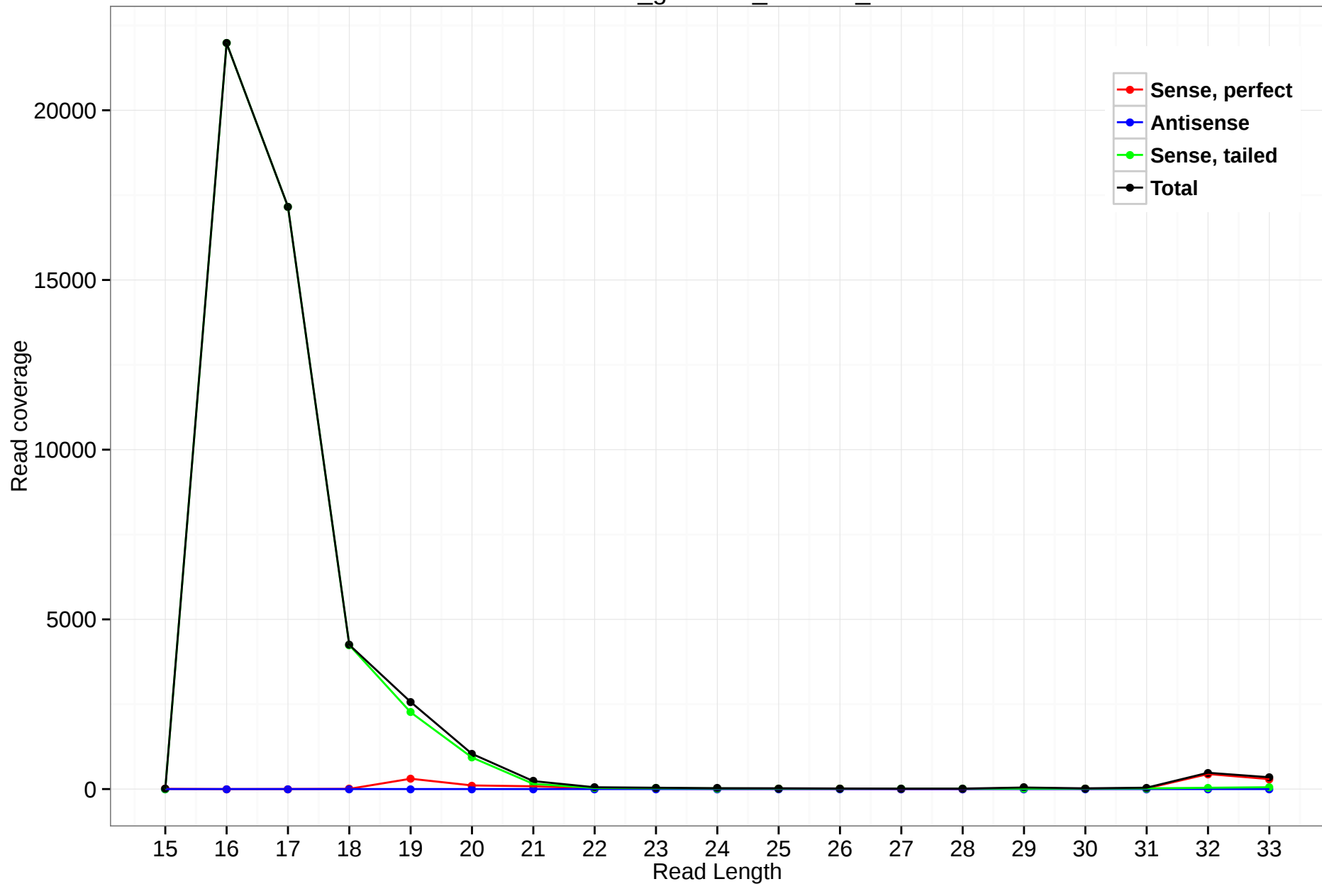
rheMac3_genscan_chr7.32_10
